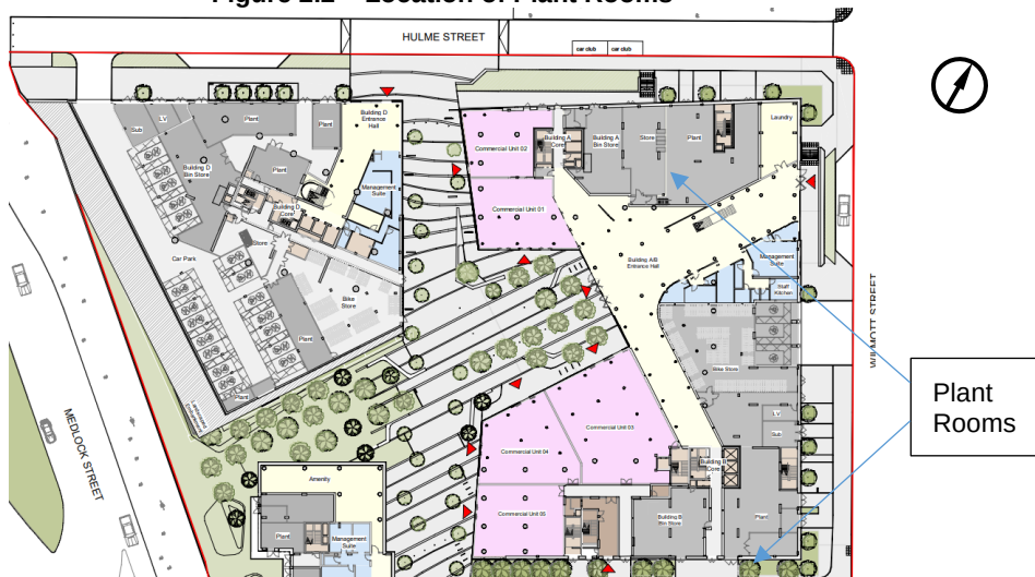
Figure 2.2 – Location of Plant Rooms
