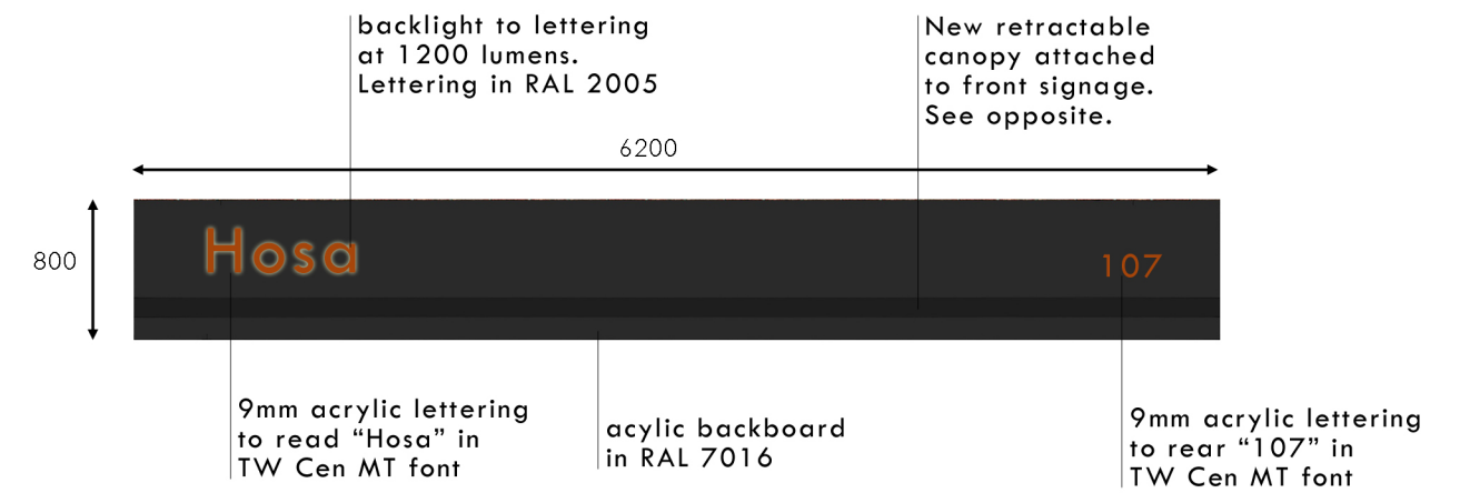
Proposed Signage Scale 1:50
