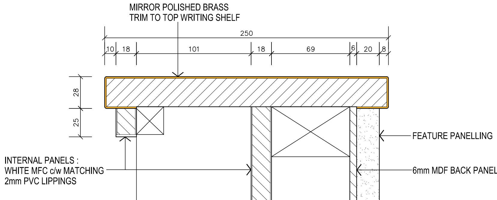
DETAIL A (1:2)
