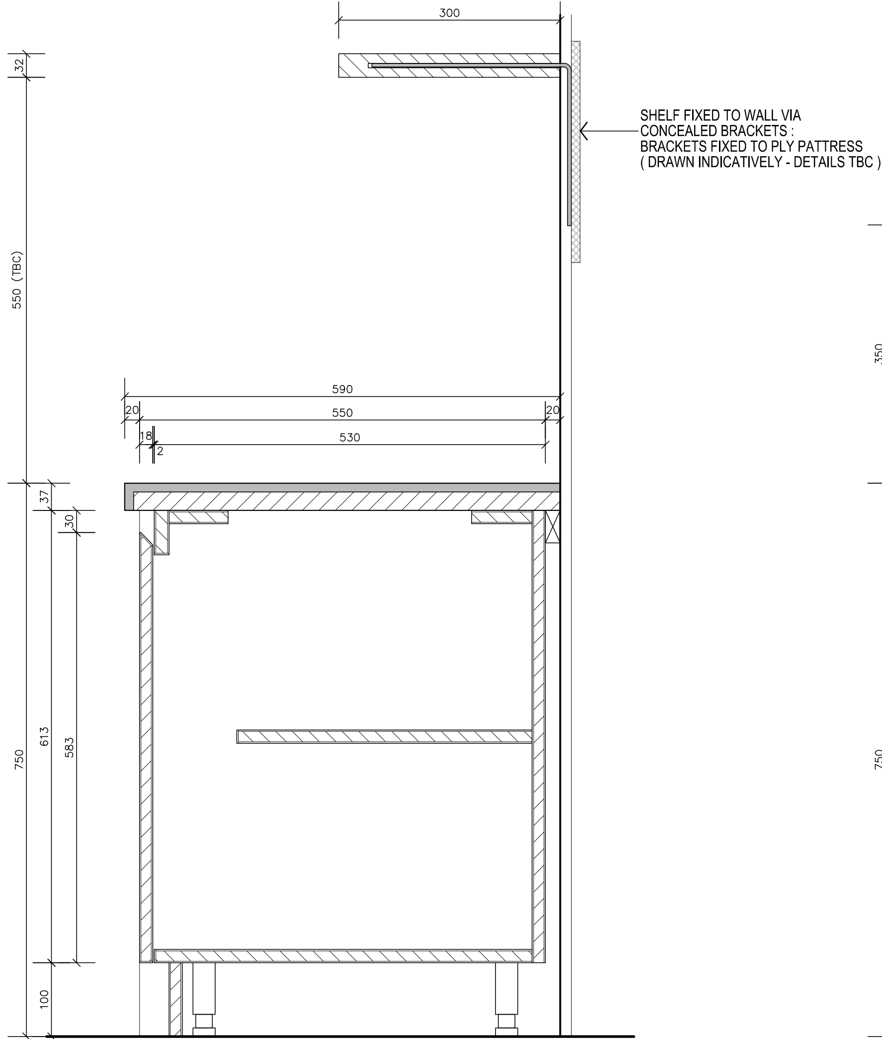
SECTION J-J
