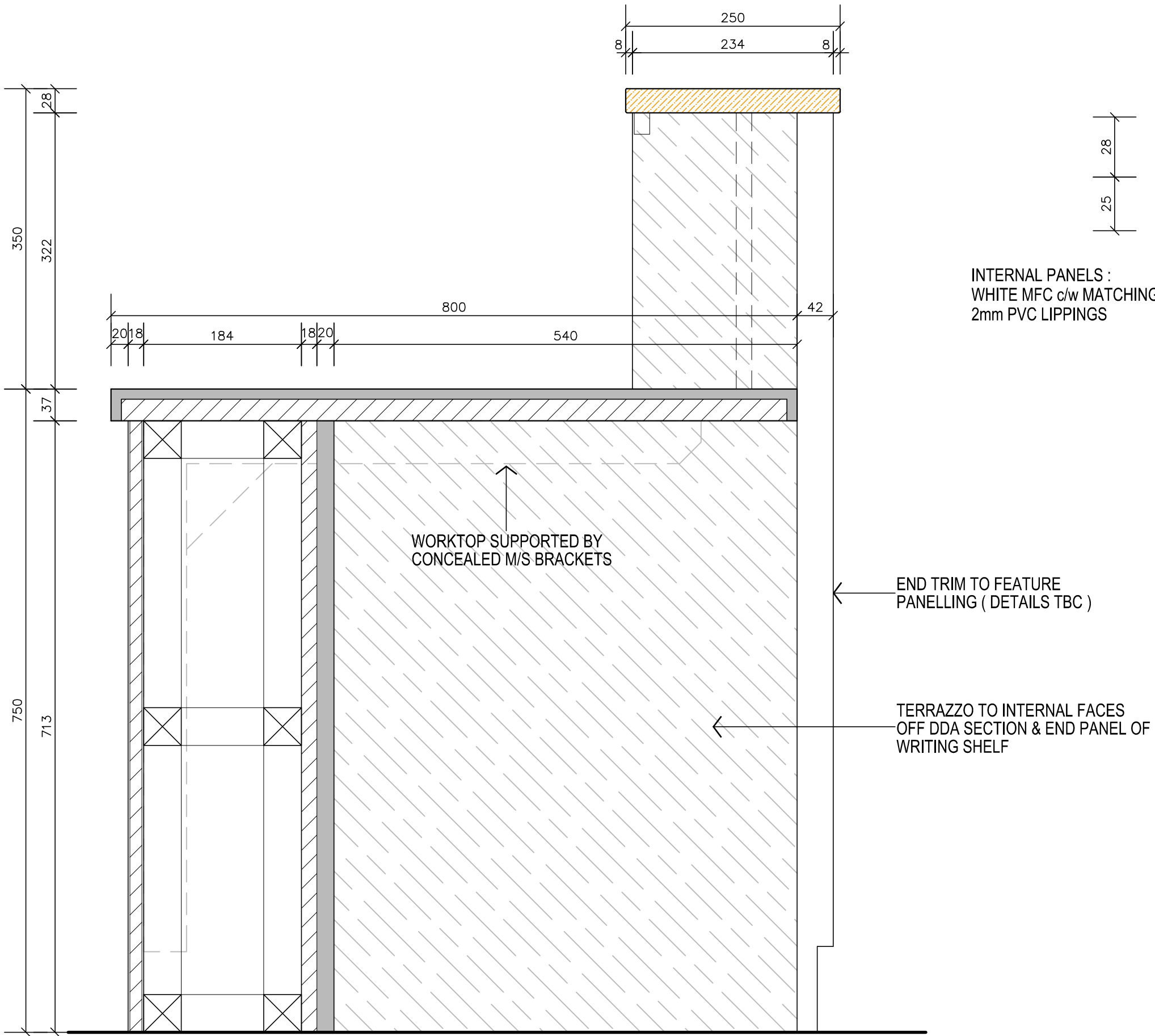
DETAIL A (1:2)
