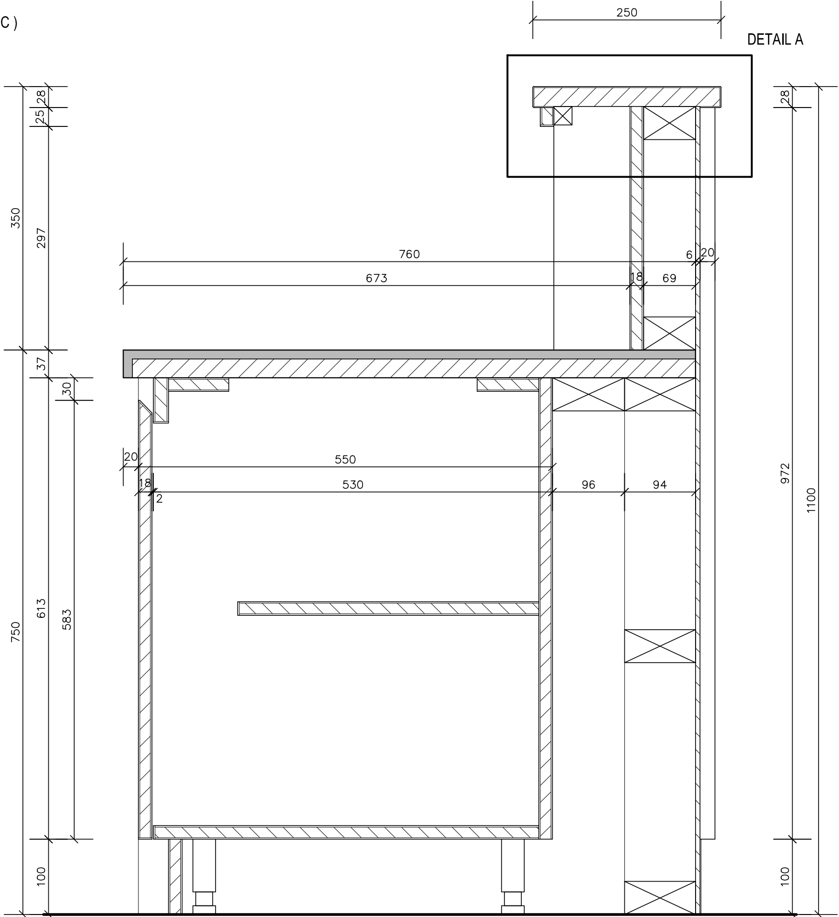
SECTION K-K
