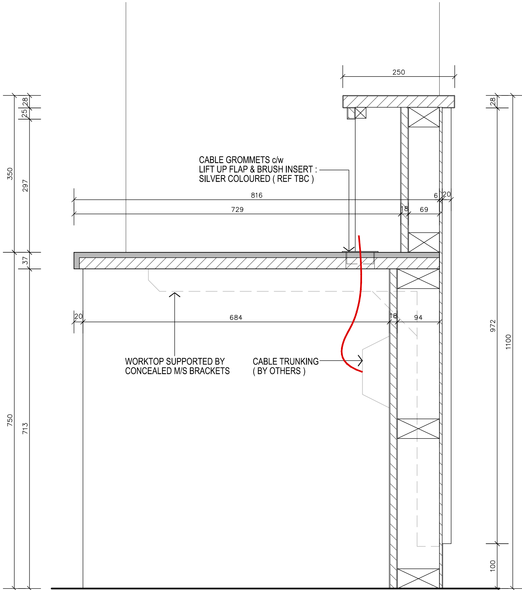
SECTION L-L
