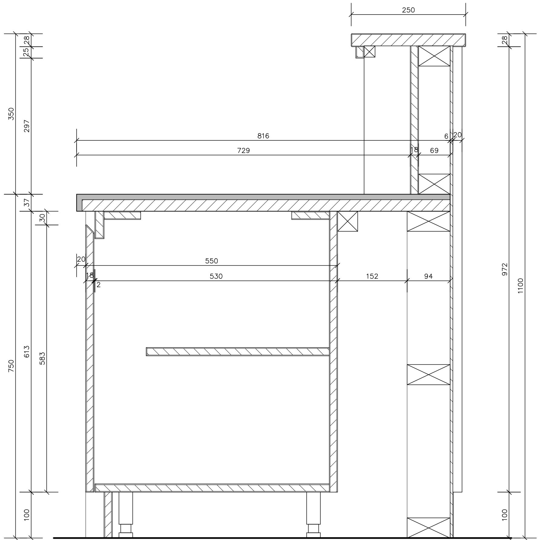
SECTION M-M
