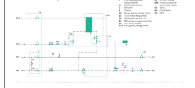
FlatStation Circuit Diagram
