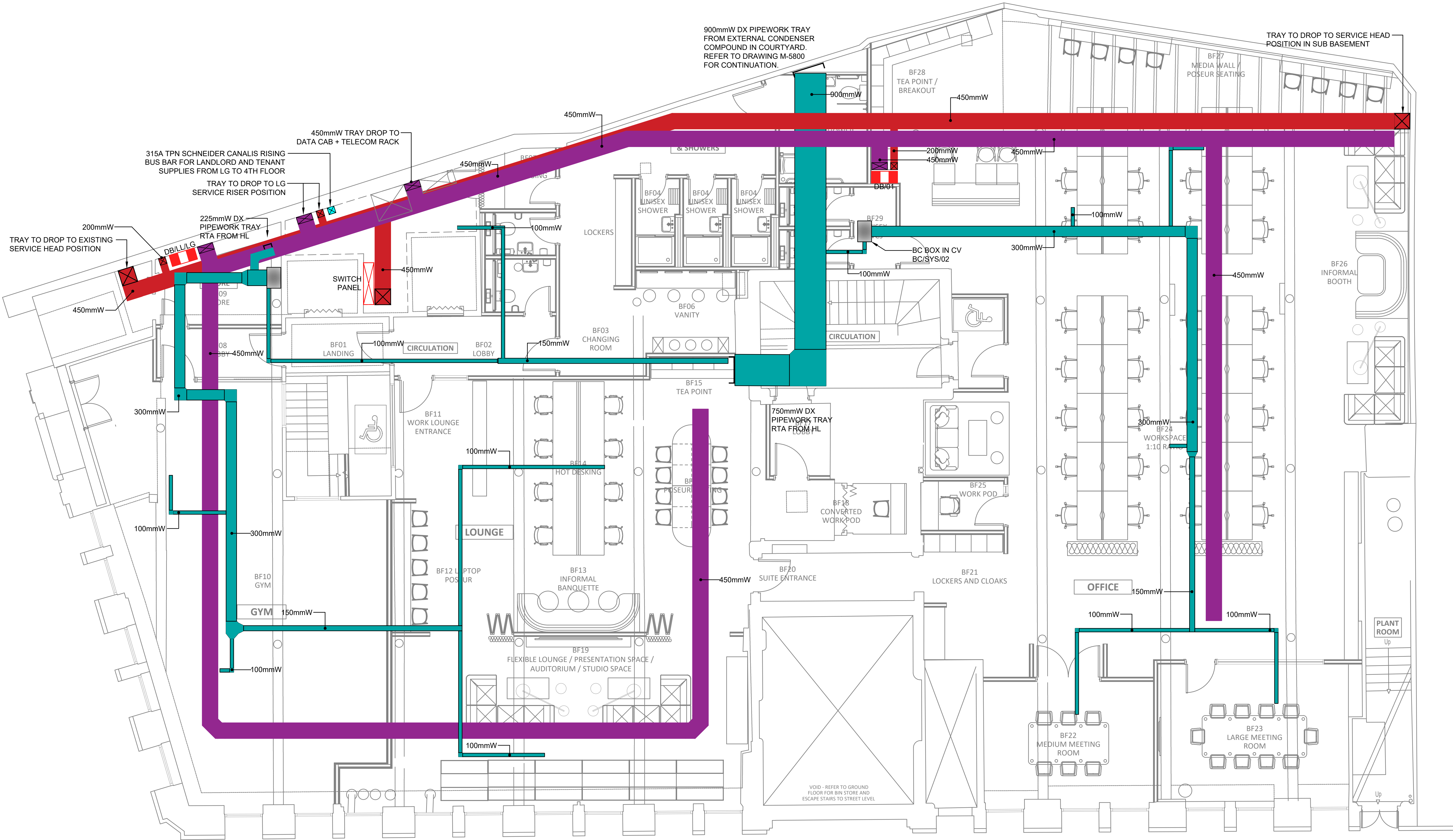
PROPOSED LOWER GROUND FLOOR
