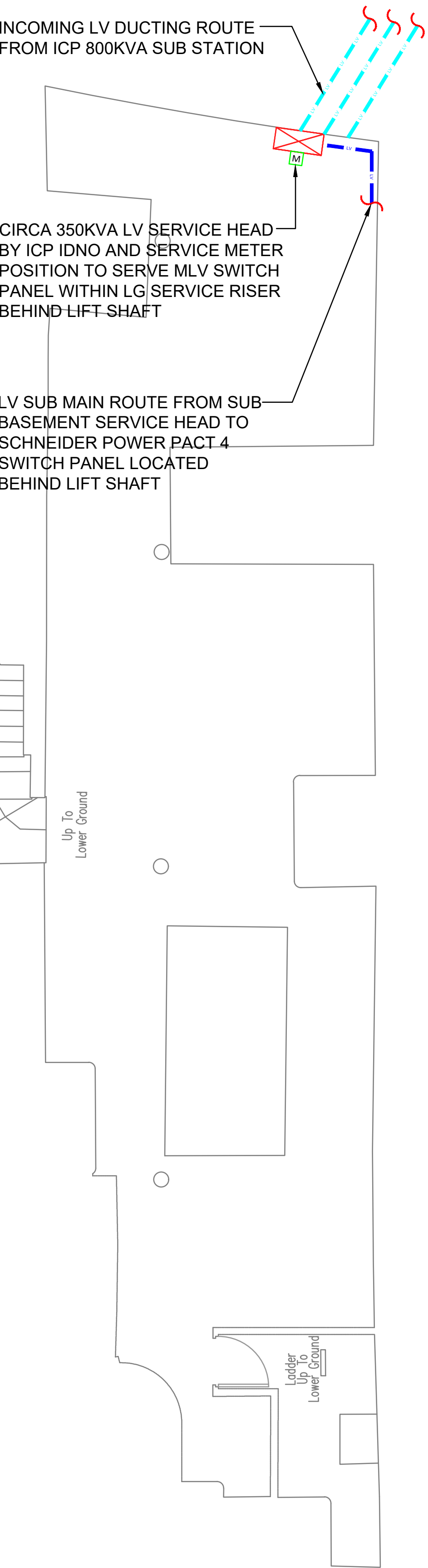
PROPOSED BASEMENT LEVEL
