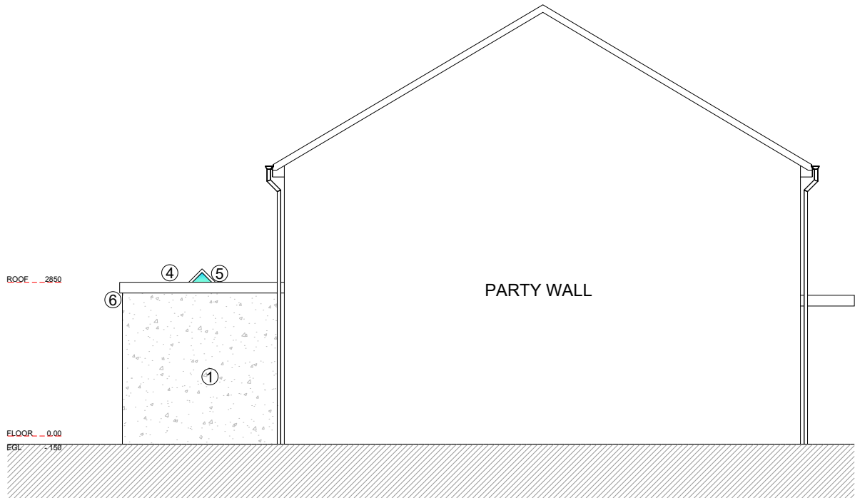
SIDE ELEVATION
