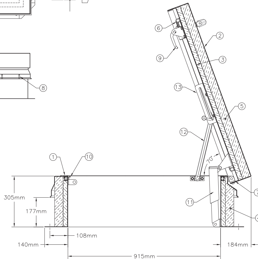
SECTION
