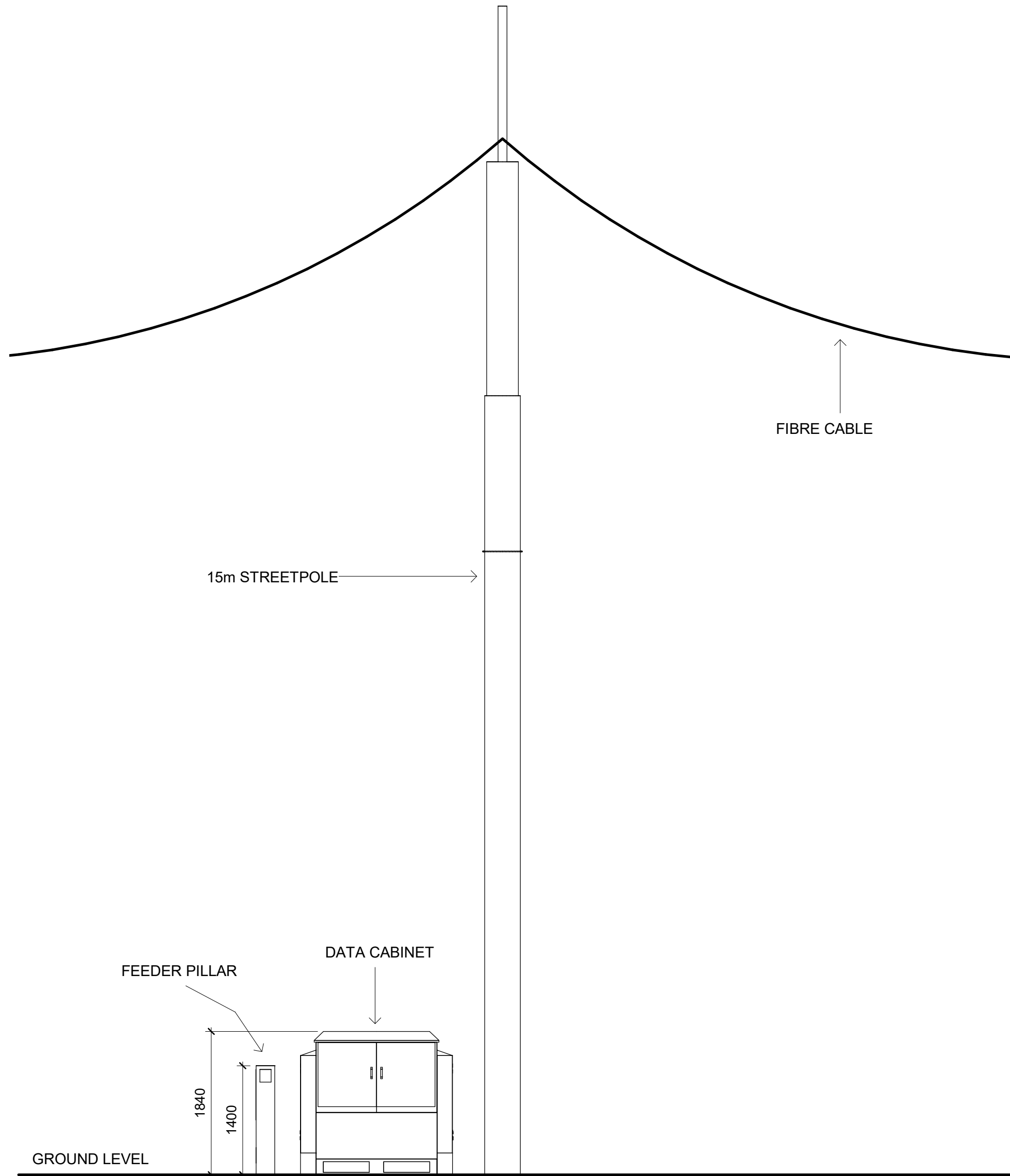
SIDE ELEVATION
