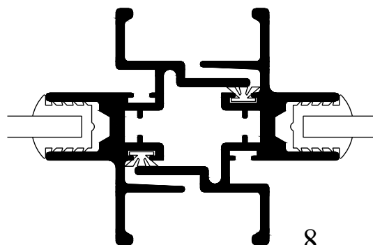
BUTT INTERLOCK
