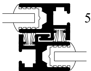
STANDARD INTERLOCK
