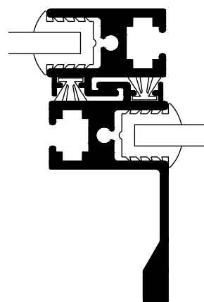
REVERSE INTERLOCK
