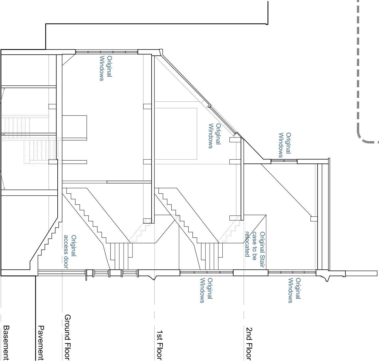
Section B
