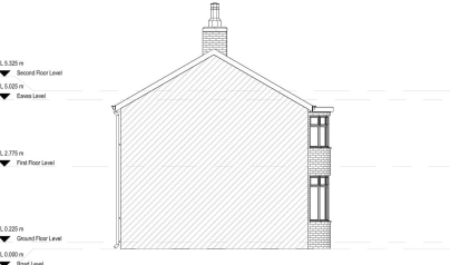
Existing Left-Side Elevation 1 : 100
