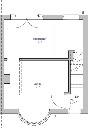
Existing Ground Floor 1 : 50
