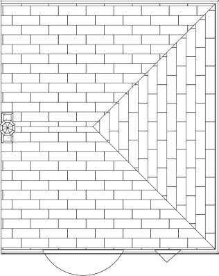
Existing Roof Plan 1 : 50
