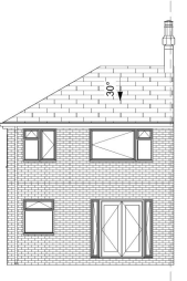
Existing Rear Elevation 1 : 100
