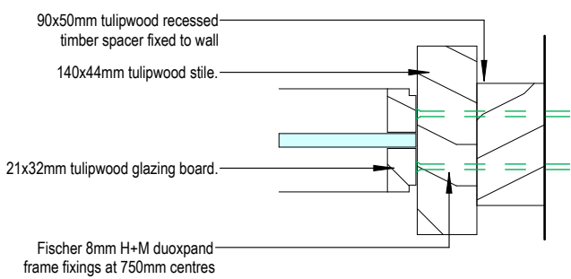
Detail C Abutment
