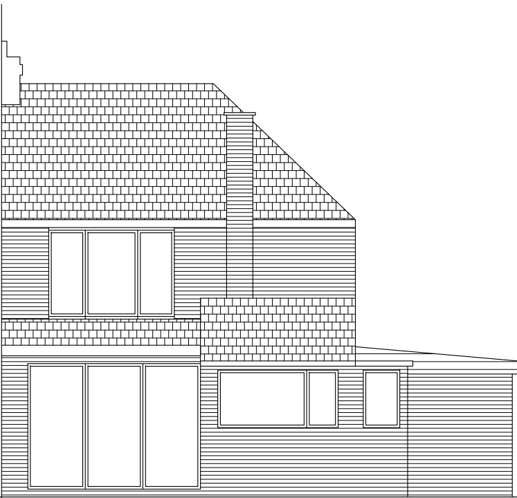
Rear Elevation
