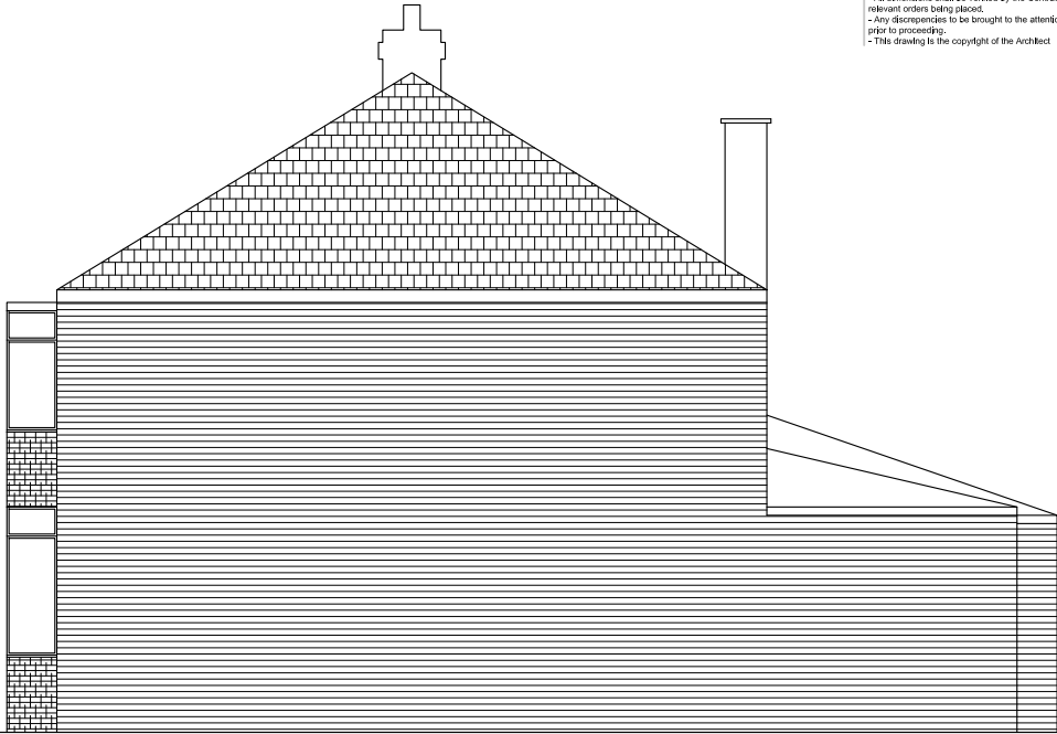
Side Elevation 02
