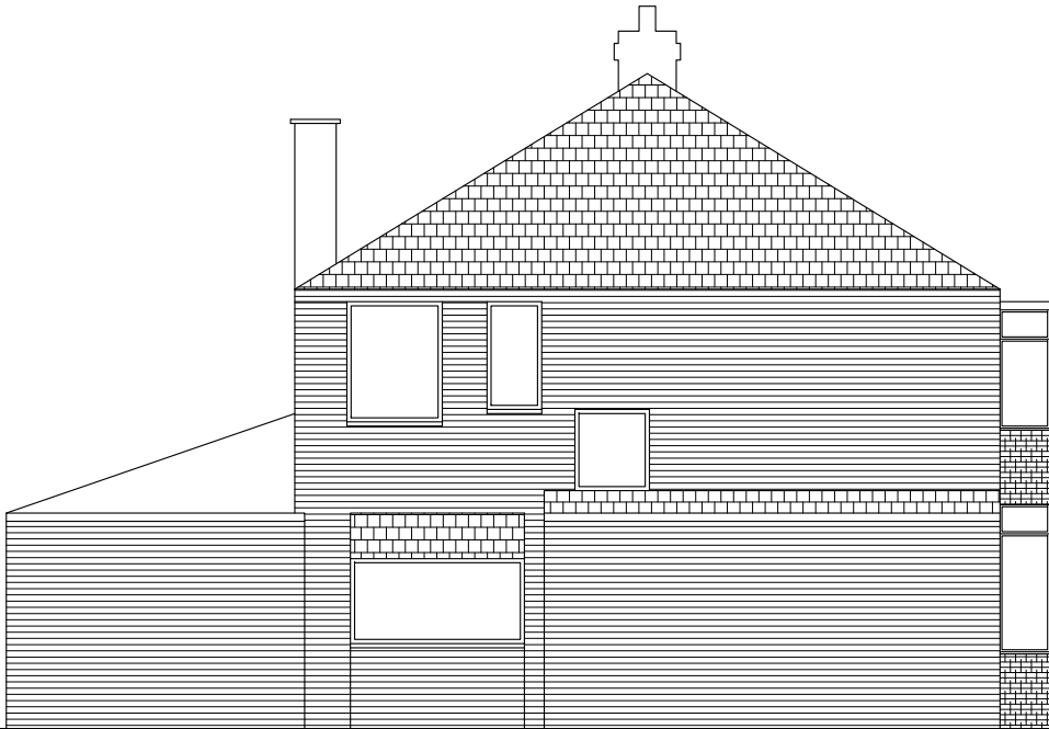
Side Elevation 01
