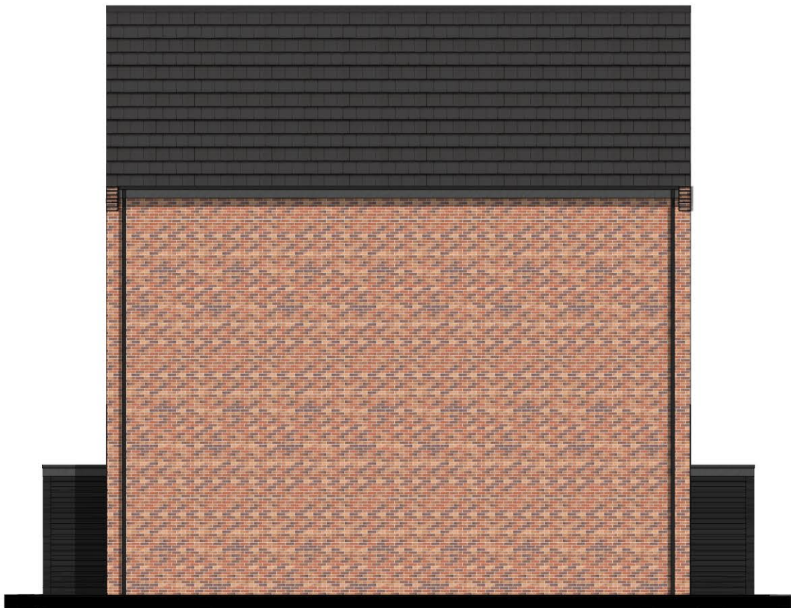
SIDE ELEVATION
