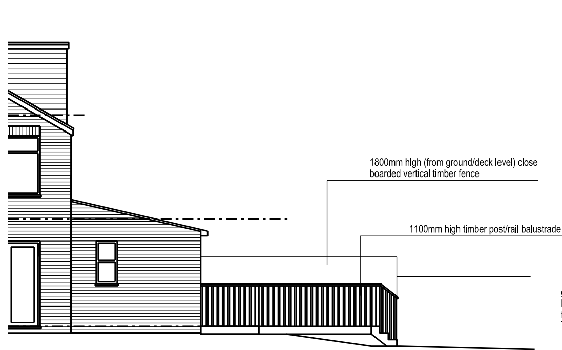
North Elevation Boundary Extract
