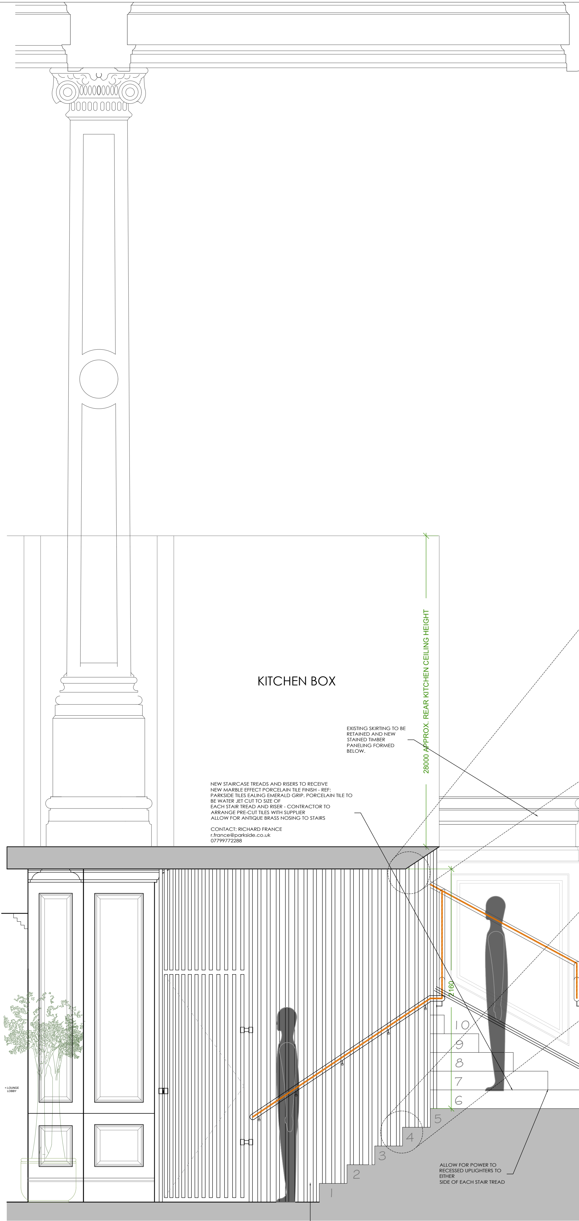
ELEVATION C (1) - STAIRS 1-9 SHOWING ONLY SCALE: 1:20 @ A1
