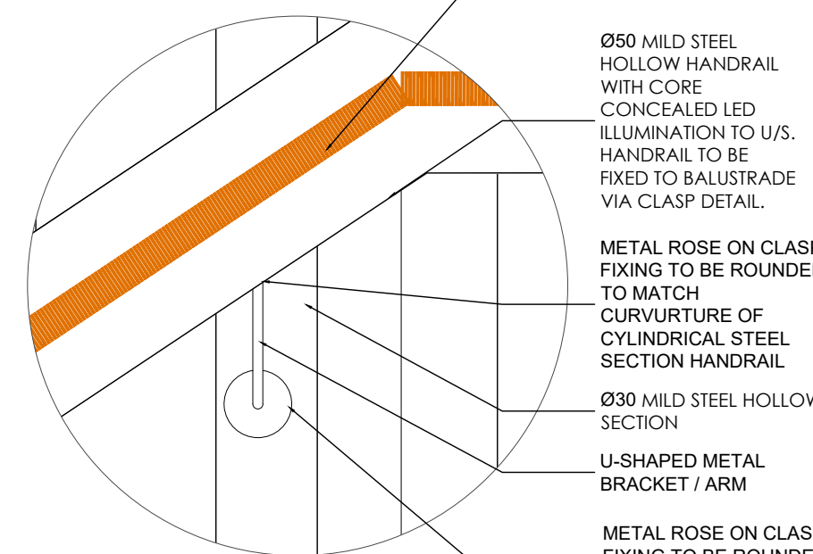
DETAIL D - FRONT VIEW SCALE 1:2 @ A1
