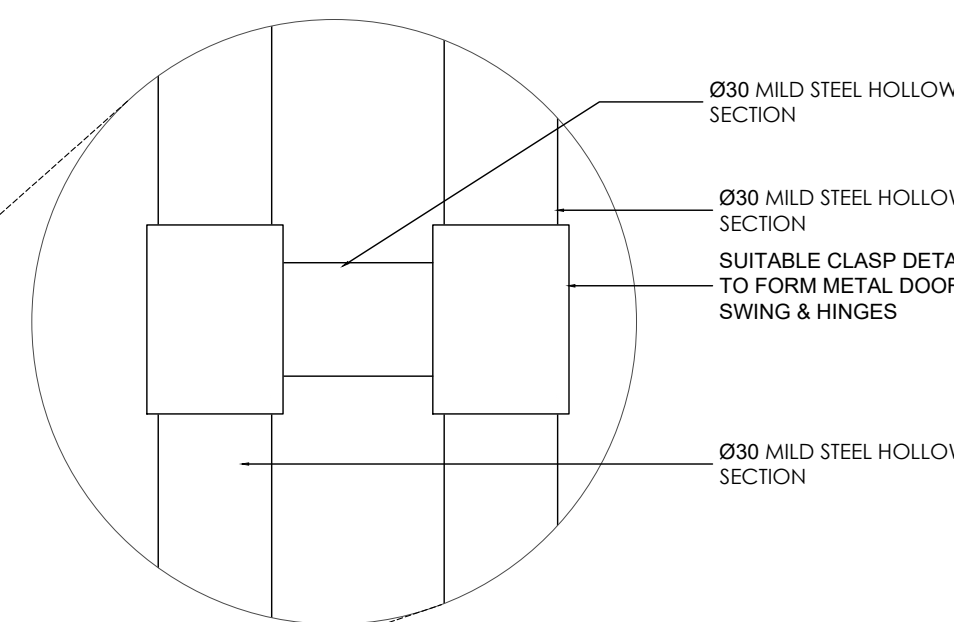
DETAIL E SCALE 1:2 @ A1
