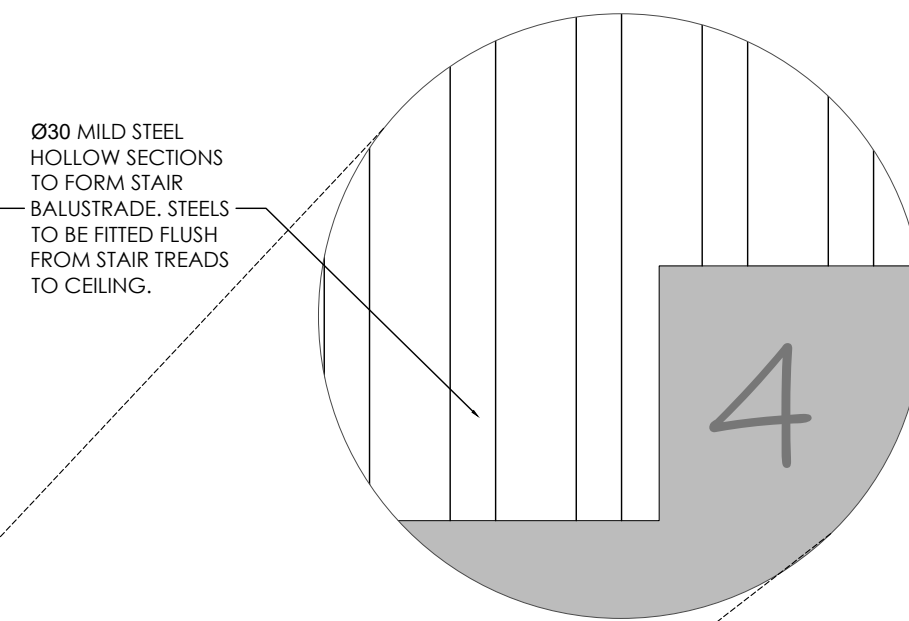
DETAIL C - STAIR TREAD SCALE 1:5 @ A1
