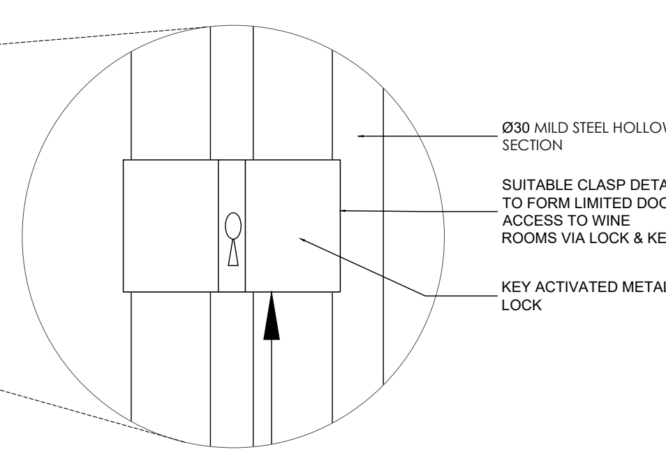
DETAIL E SCALE 1:2 @ A1
