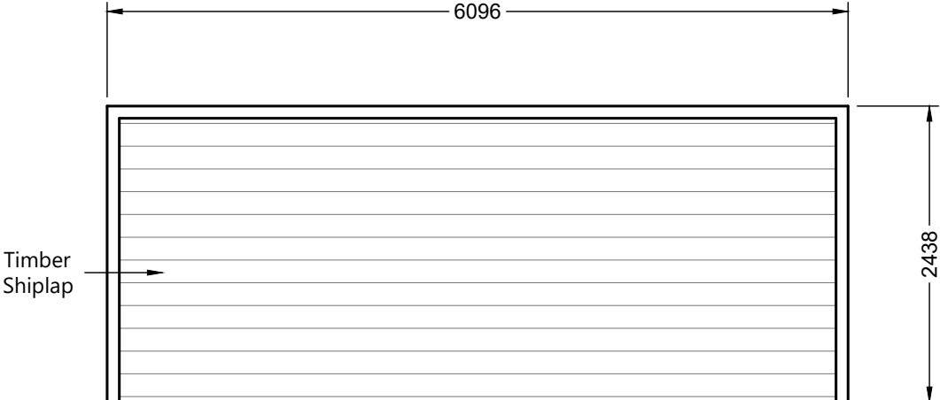
EAST ELEVATION
