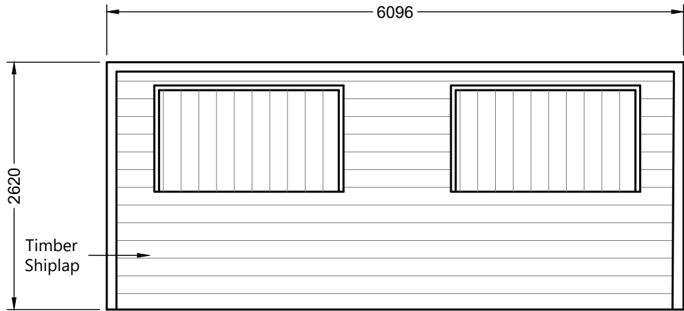
WEST ELEVATION
