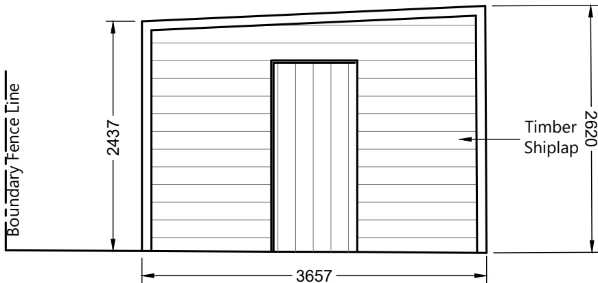
NORTH ELEVATION
