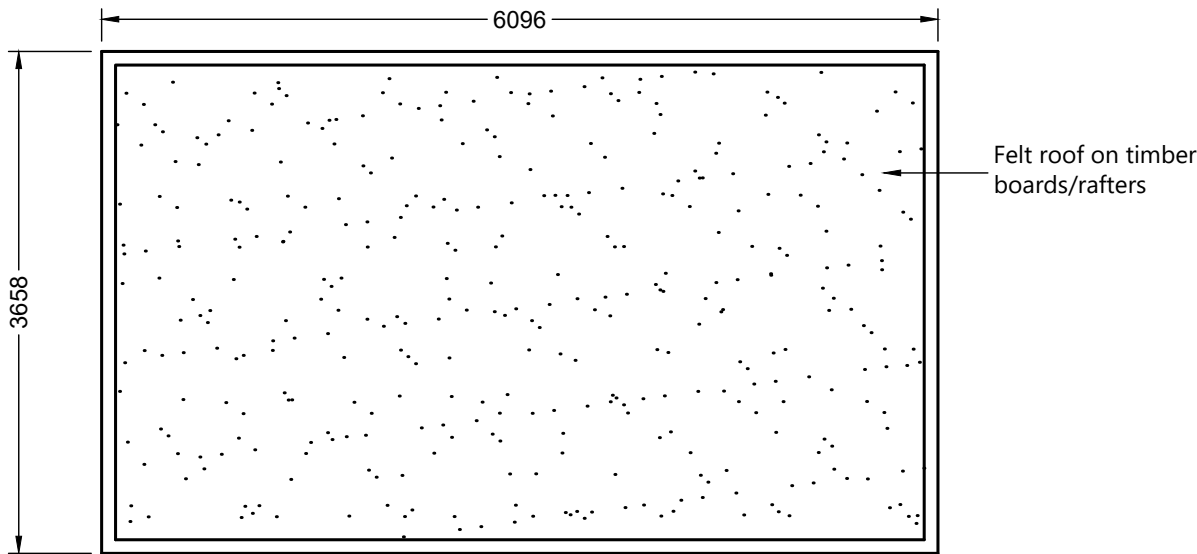
ROOF PLAN
