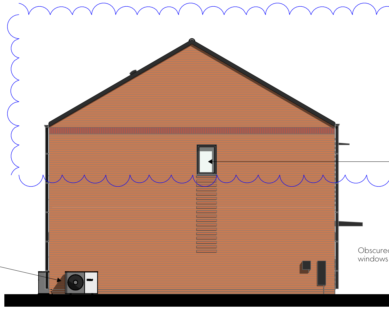
Gable Elevation - End Terrace - Plot 12 Scale @ 1:75
