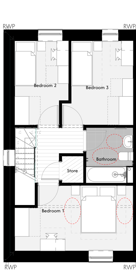
First Floor Plan Scale @ 1:75
