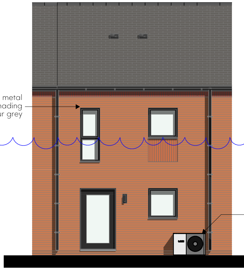
Rear Elevation - Middle Terrace Scale @ 1:75
