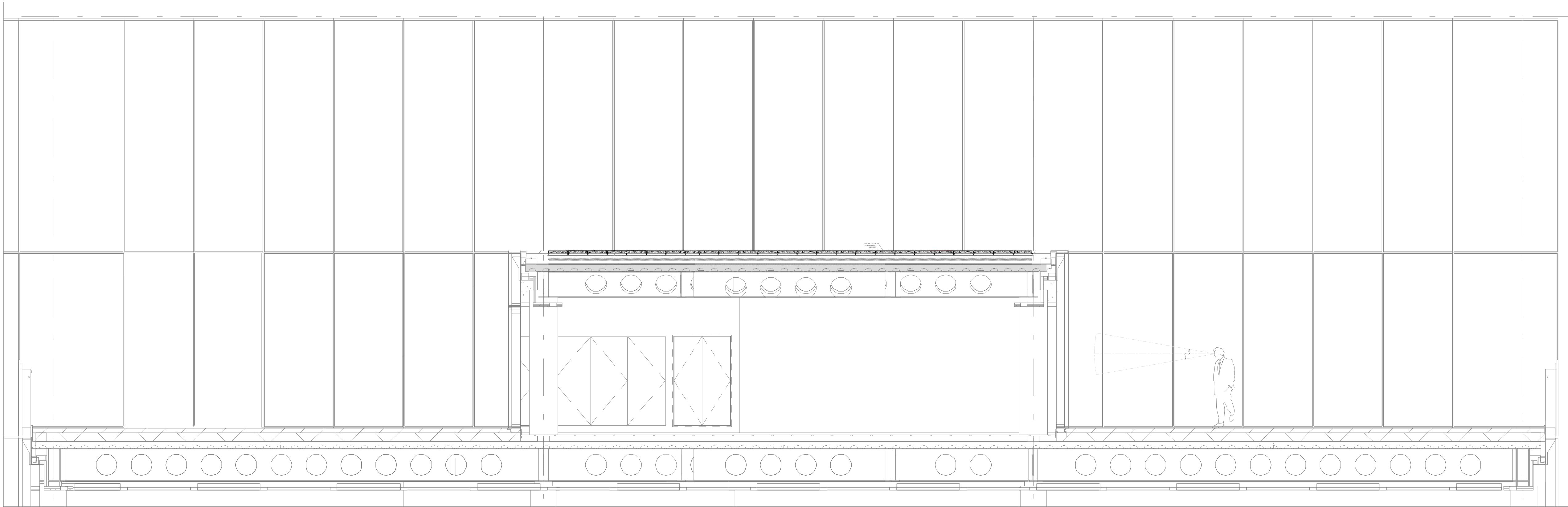
SECTION @ 1:50 SCALE
