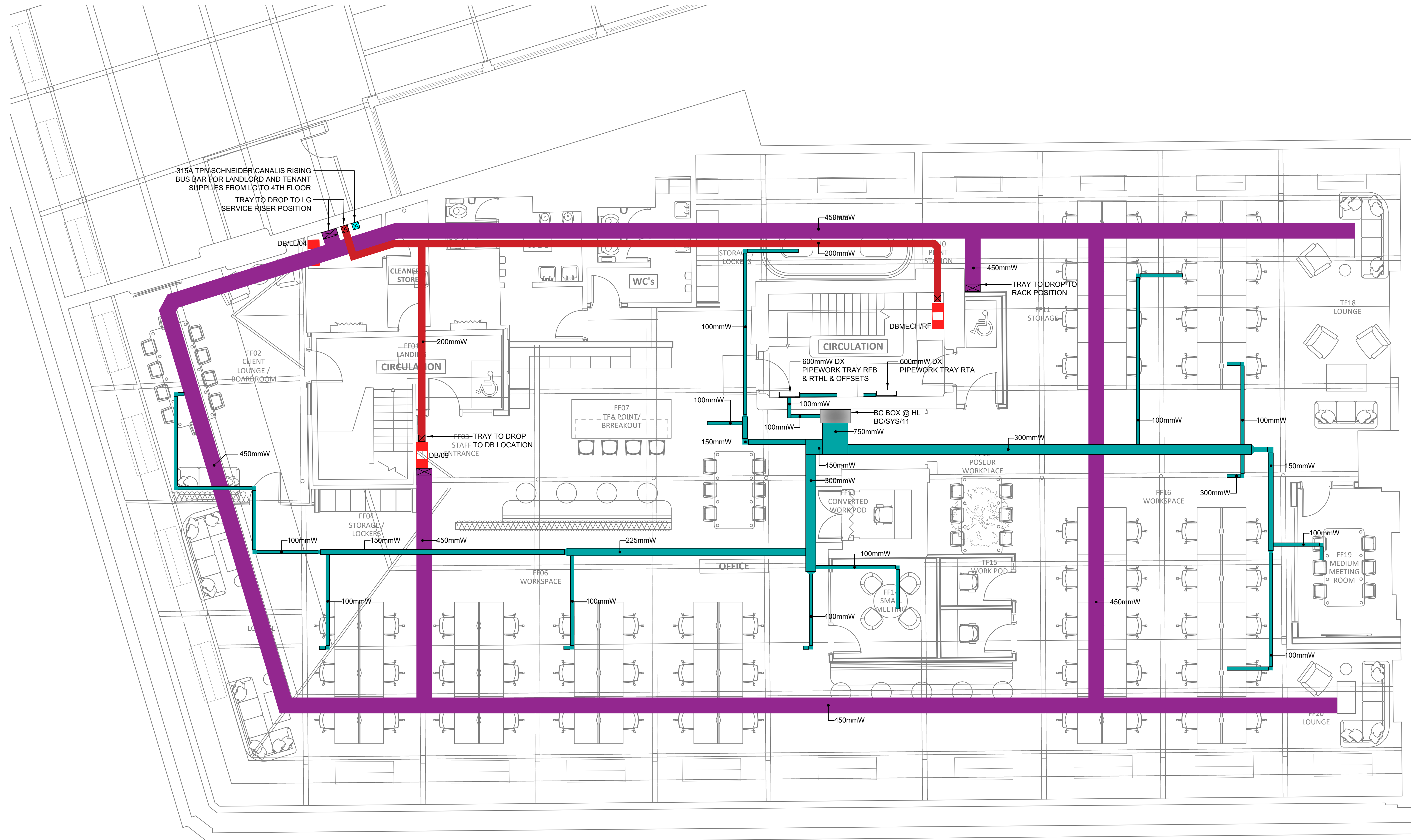
PROPOSED FOURTH FLOOR
