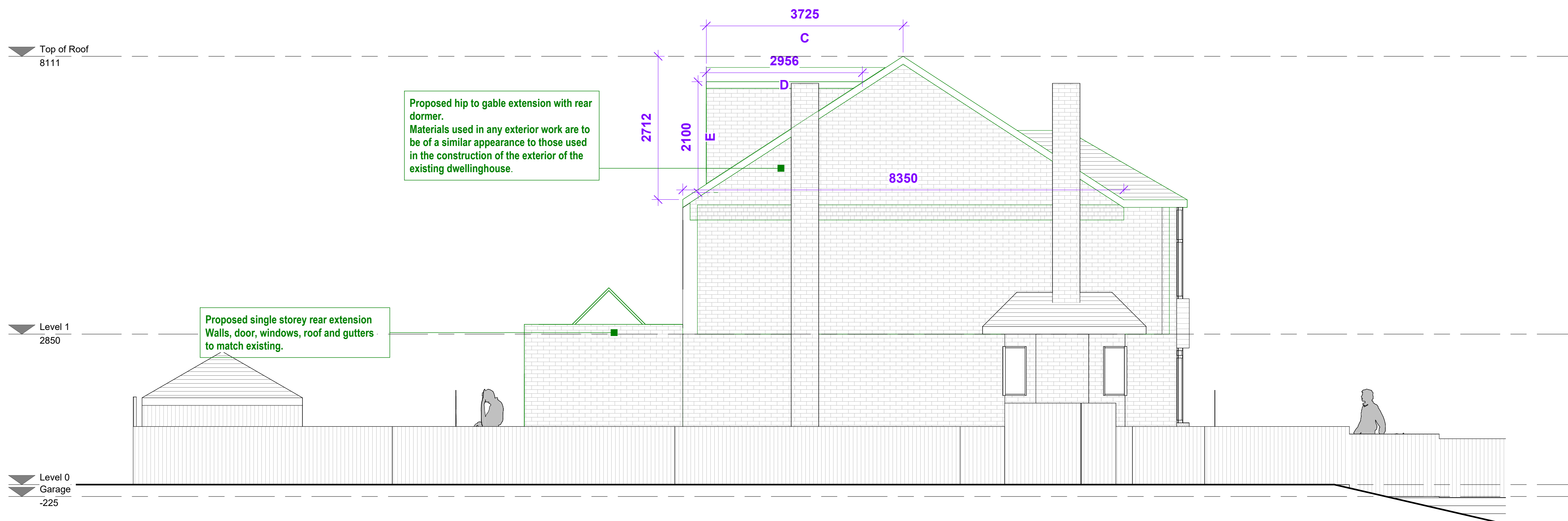
2 Proposed Side 1 Elevation 1 : 50
