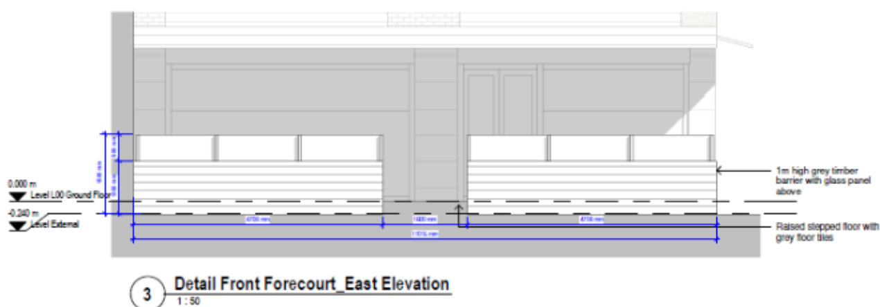
Image 1 Proposed Front (East) Elevation
