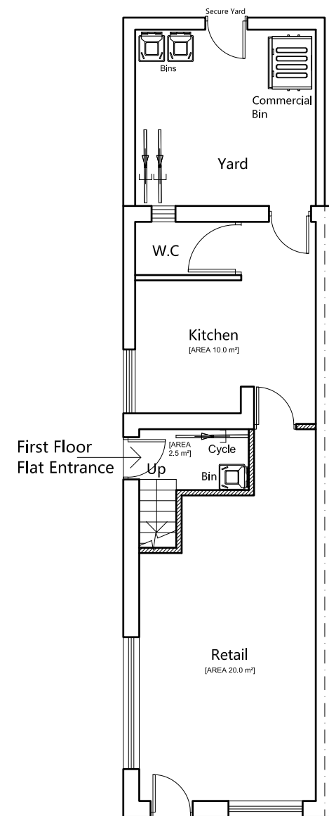
Proposed Ground Floor Plan
