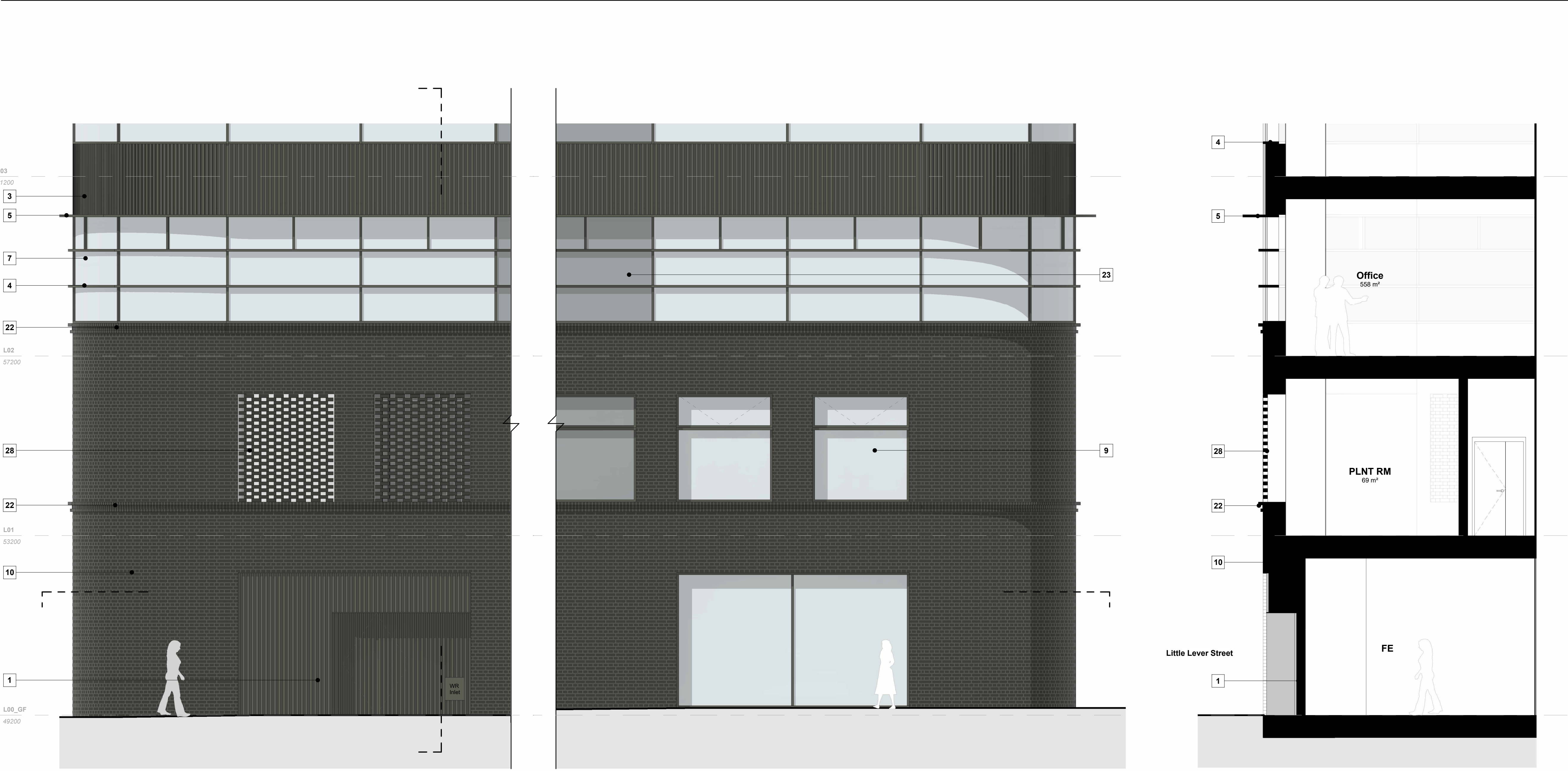
Typical Bay Study 03 - Elevation 1:50
