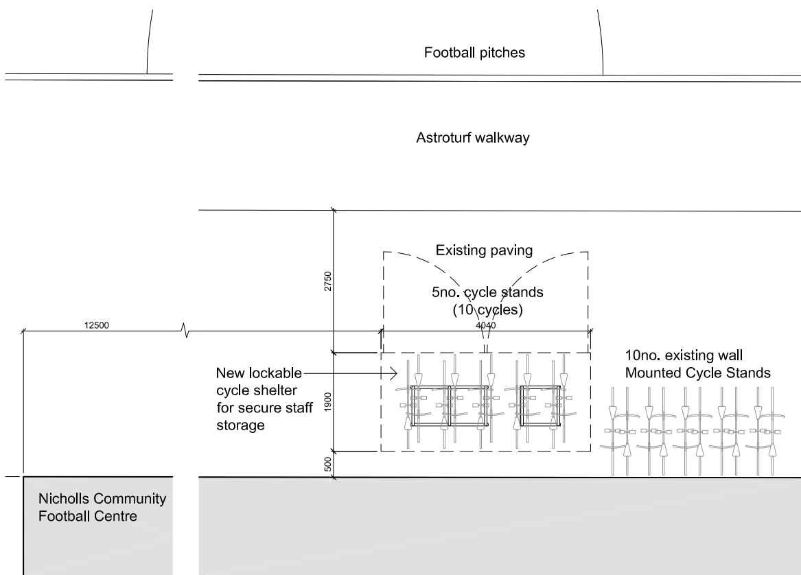
CYCLE STORAGE PLAN 1:100 @ A3
