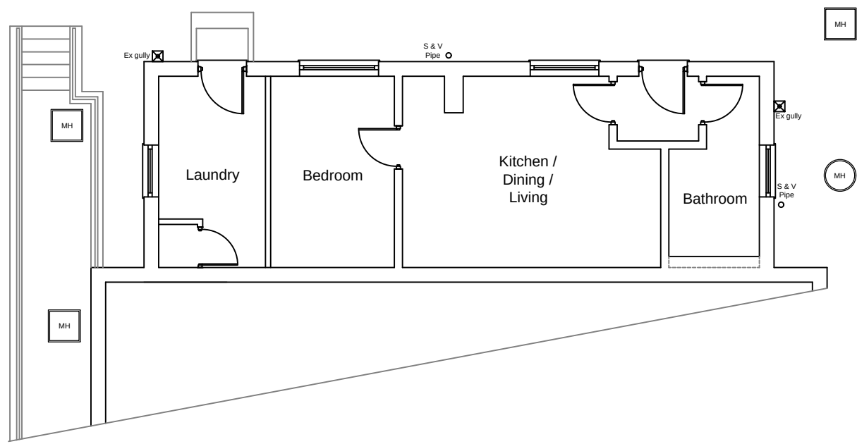
Existing Lower Ground Floor Plan
