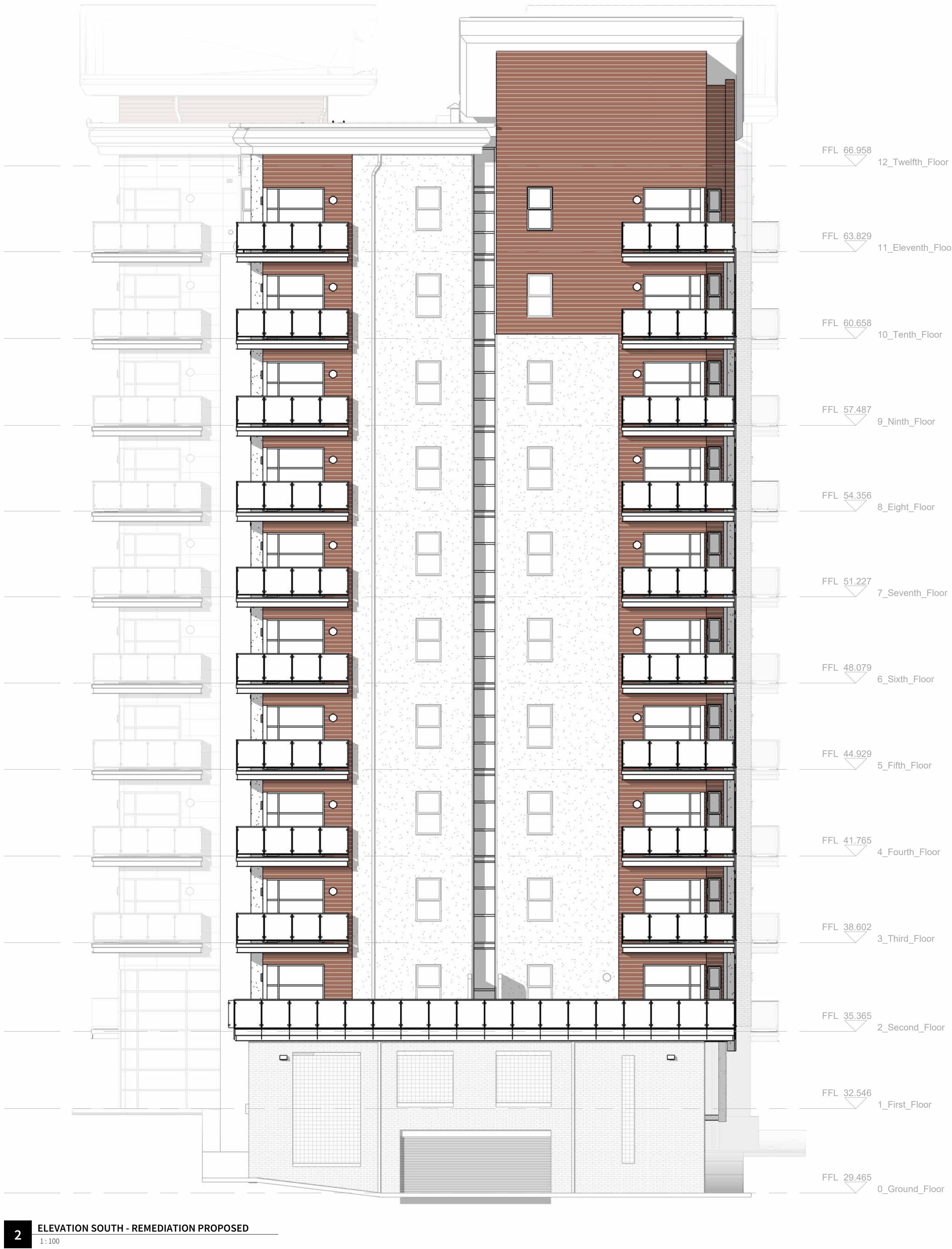
2 ELEVATION SOUTH - REMEDIATION PROPOSED 1:100
