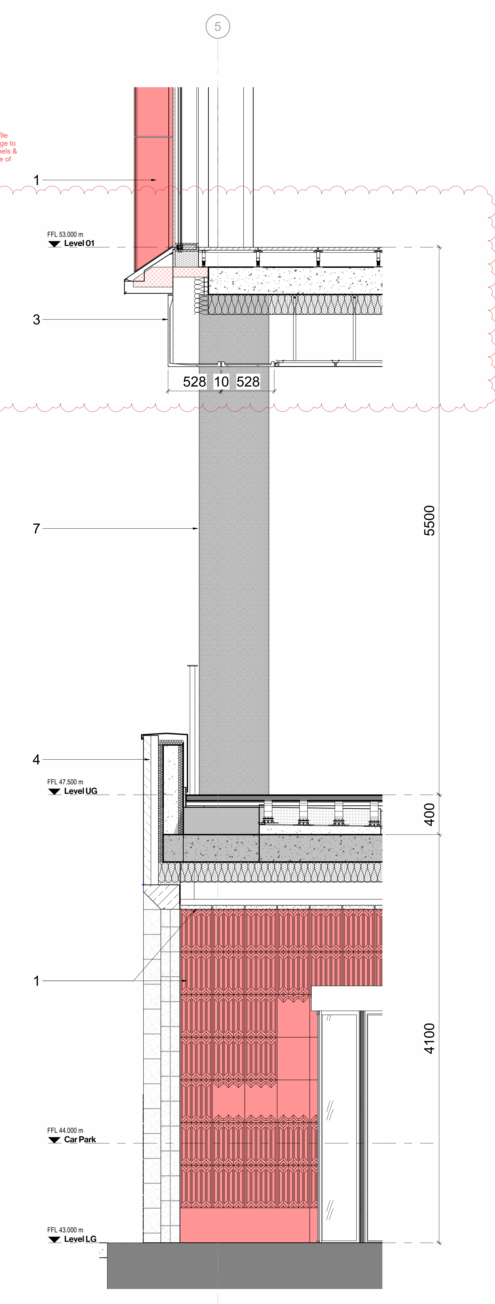
2 Lower Ground Bay Study - Section
