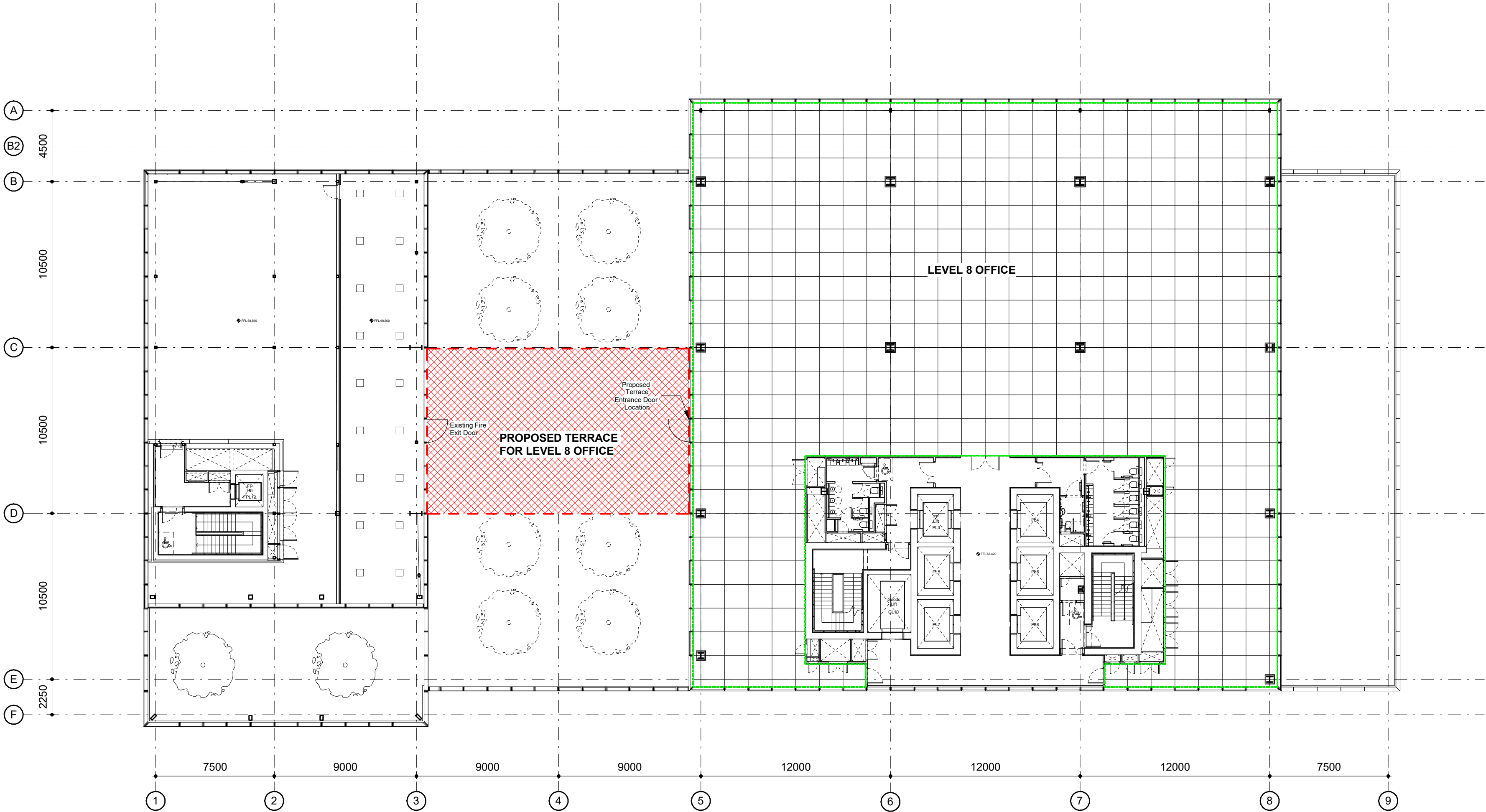
Eight Floor - Demise Area Plan 1 : 200
