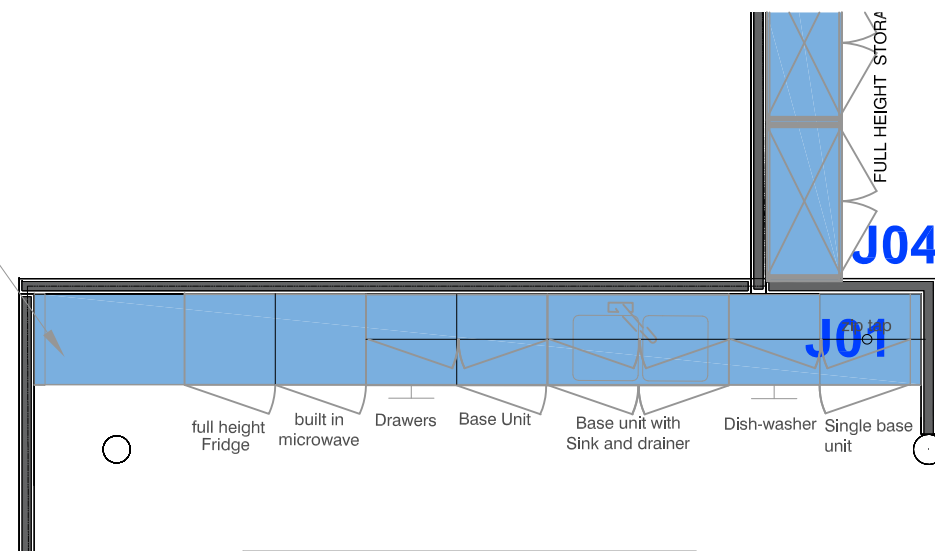
Plan View Scale 1/50
