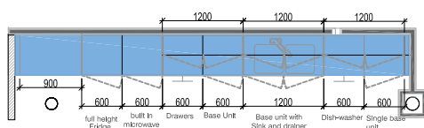
J01. Kitchen - Suite 1 Scale 1/100
