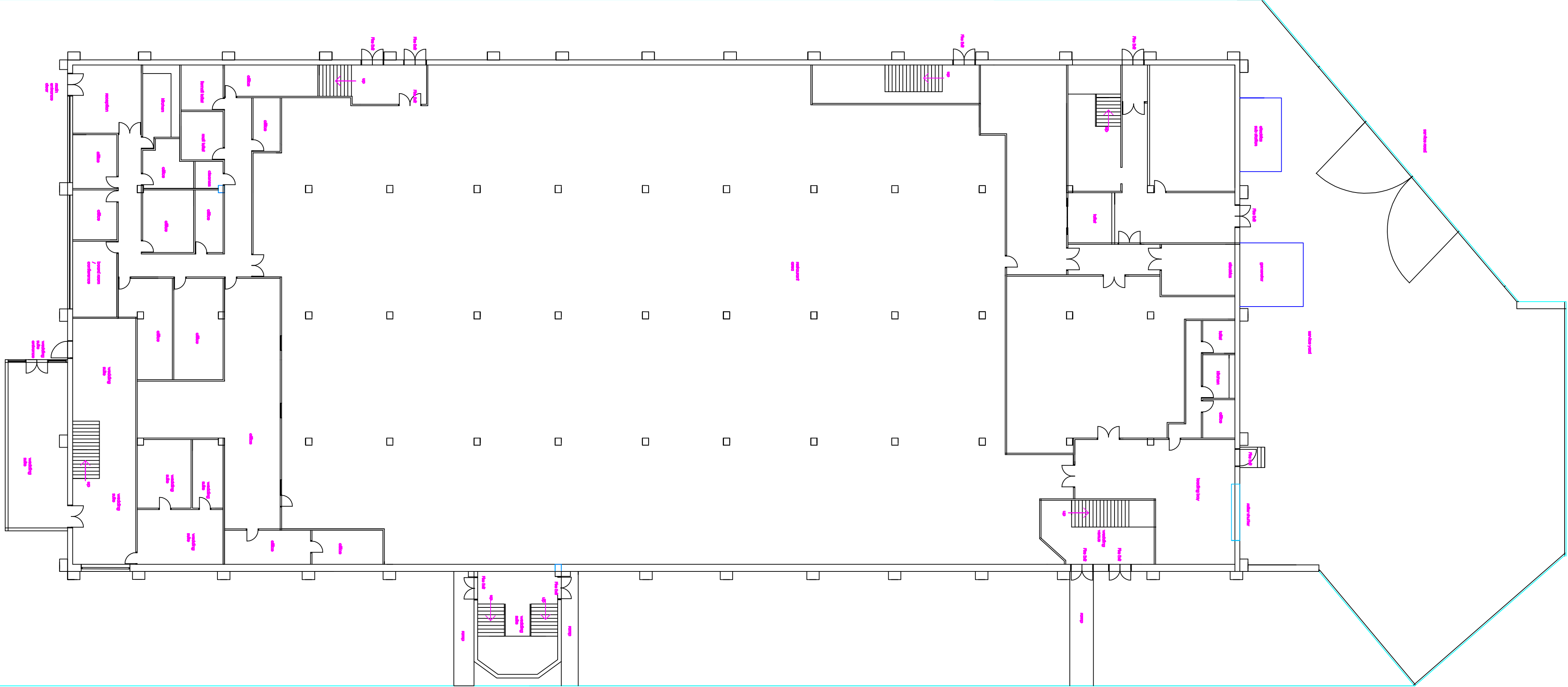
EXISTING GROUND FLOOR SCALE 1:200
