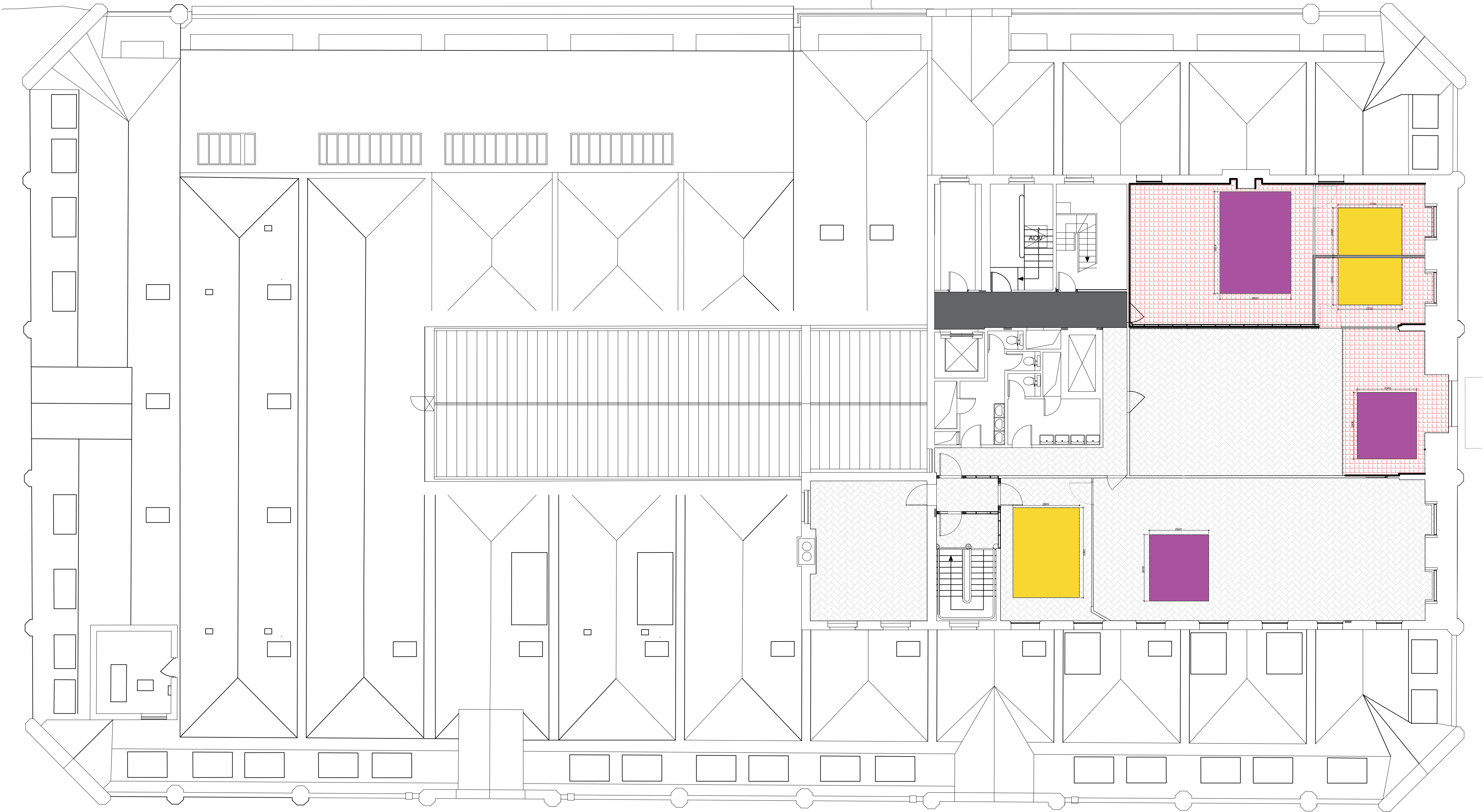
Floor Finishes - Fifth Floor Scale 1:100
