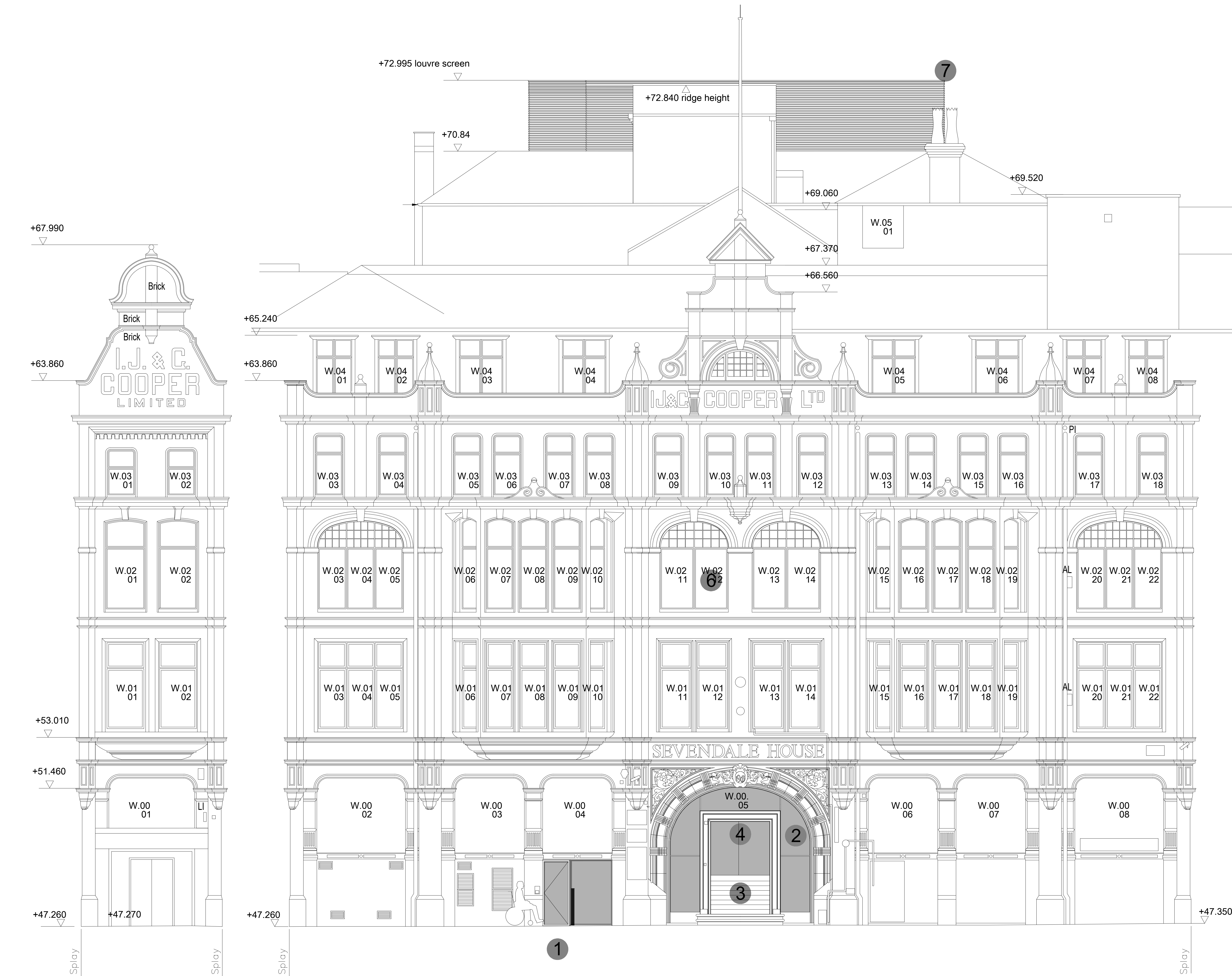
Dale Street Elevation Scale 1:50
