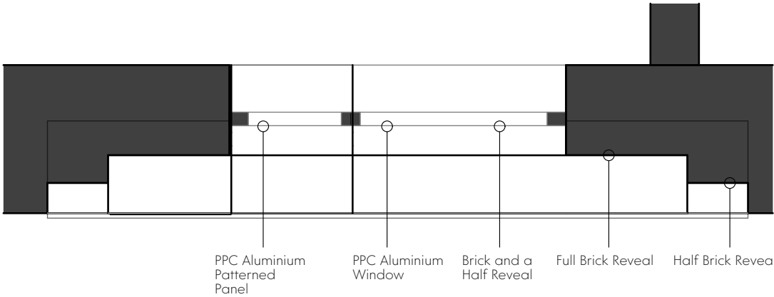
Typical Window Plan - 1:20@A3
