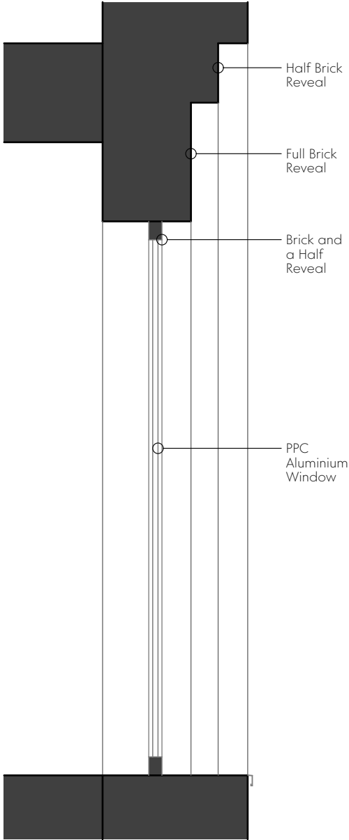
Typical Window Section - 1:20@A3
