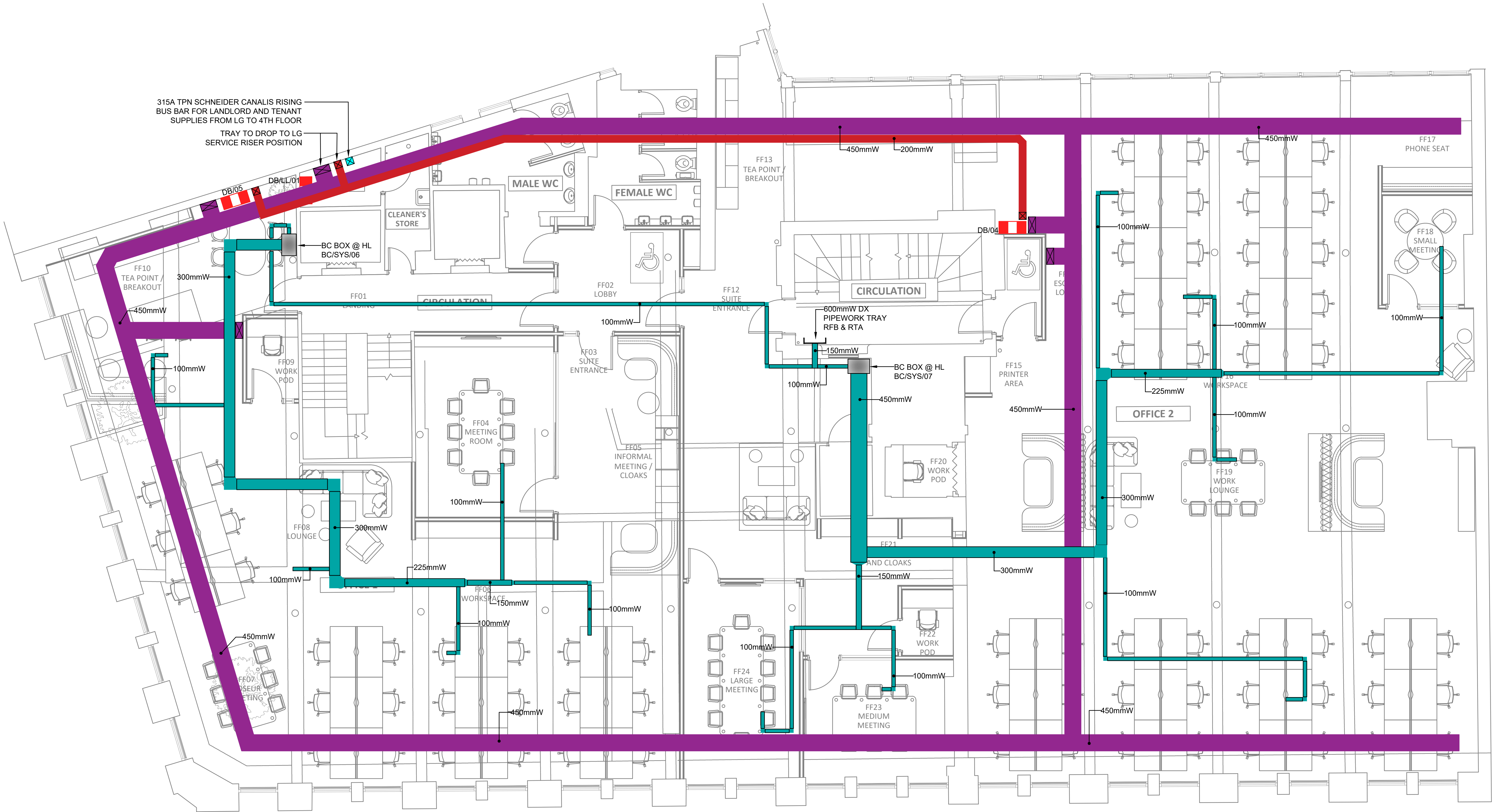
PROPOSED FIRST FLOOR
