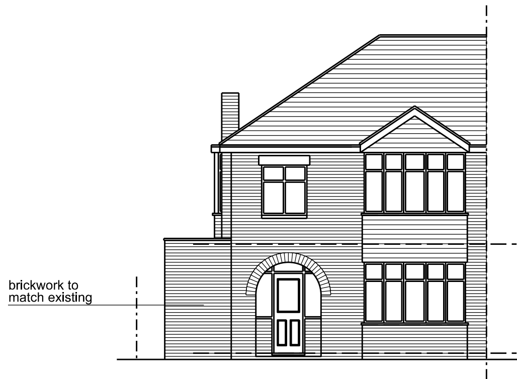
West Elevation
