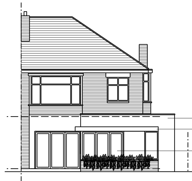
East Elevation
