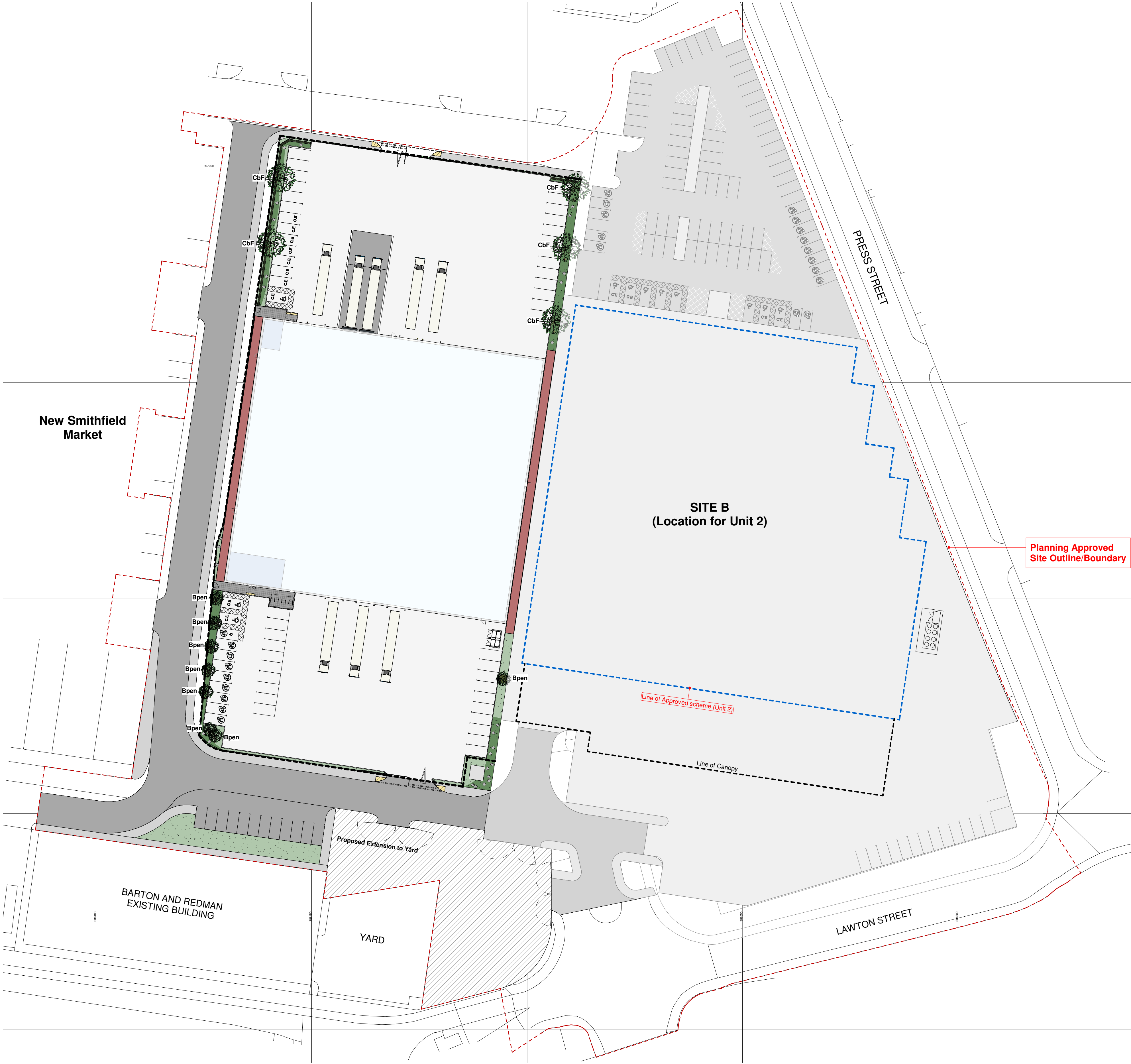
1 Landscape Masterplan- Hard/Soft Landscape Finishes 1 : 500
