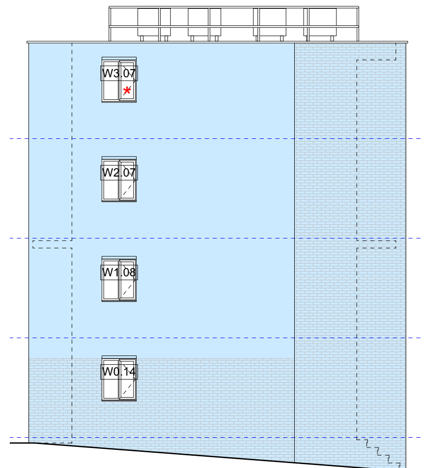
SOUTH ELEVATION
