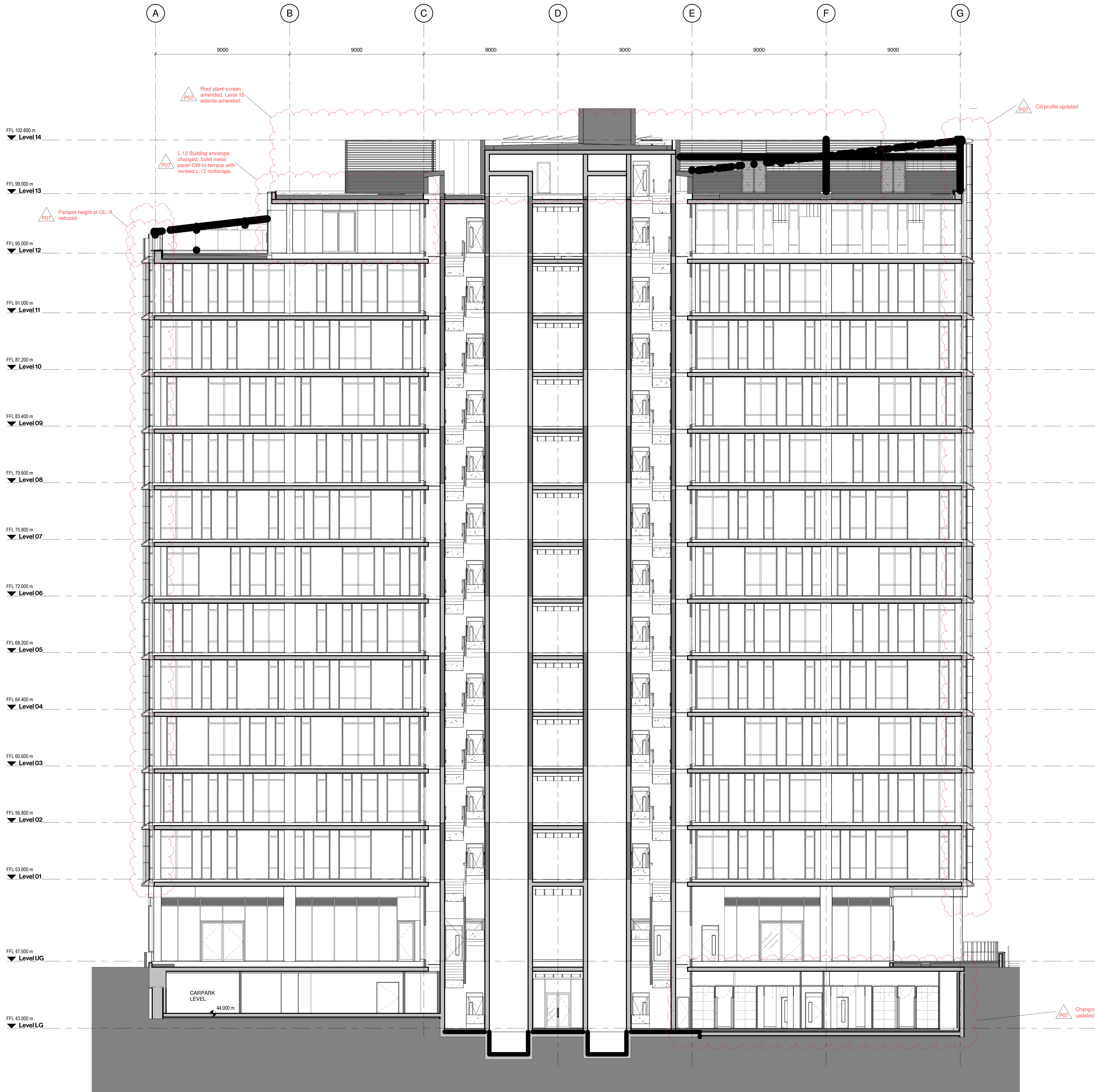
1 Section - AA
