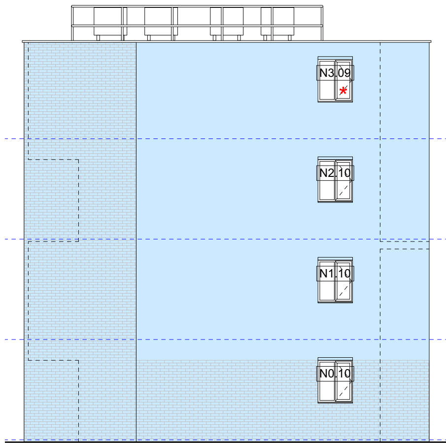
EAST ELEVATION
