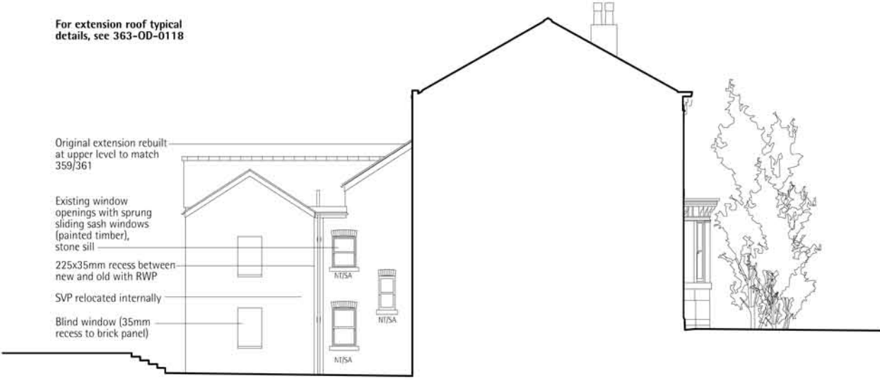
NE Elevation (As Proposed) 1:100
