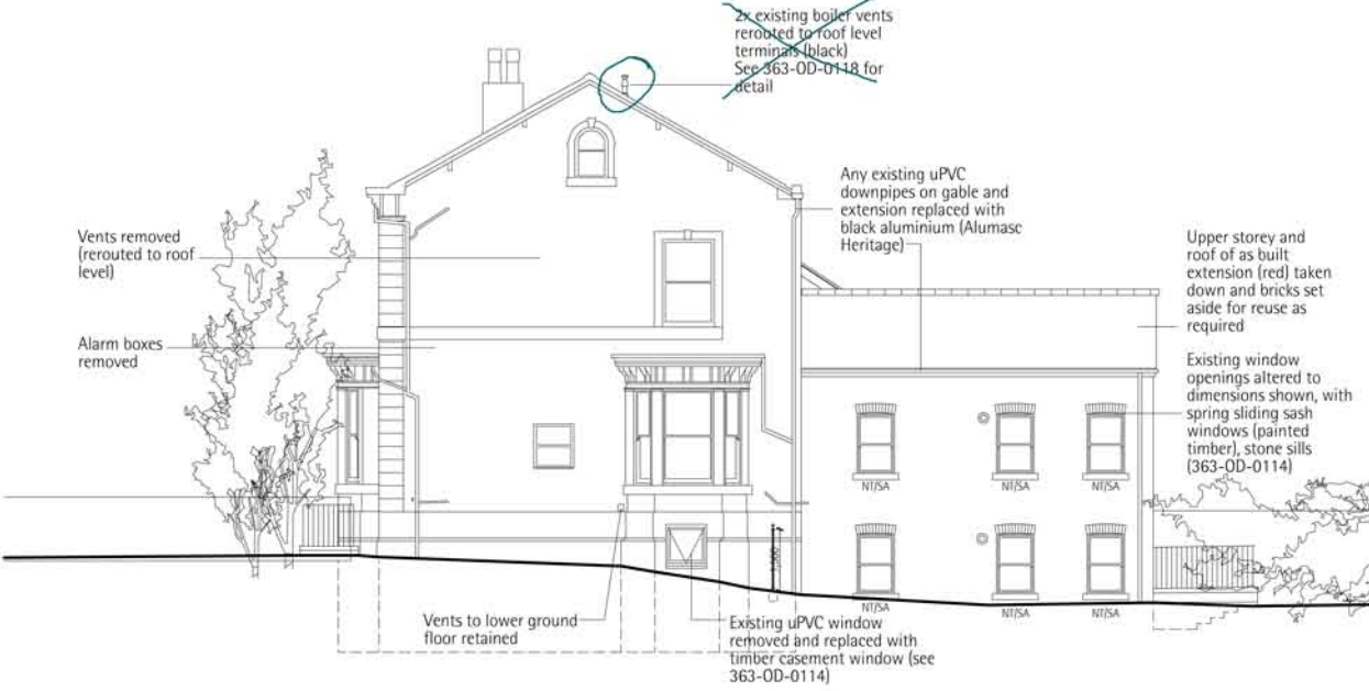
SW Elevation (As Proposed) 1:100
