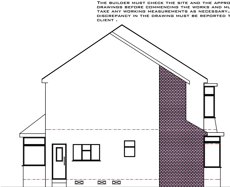
Side Elevation
