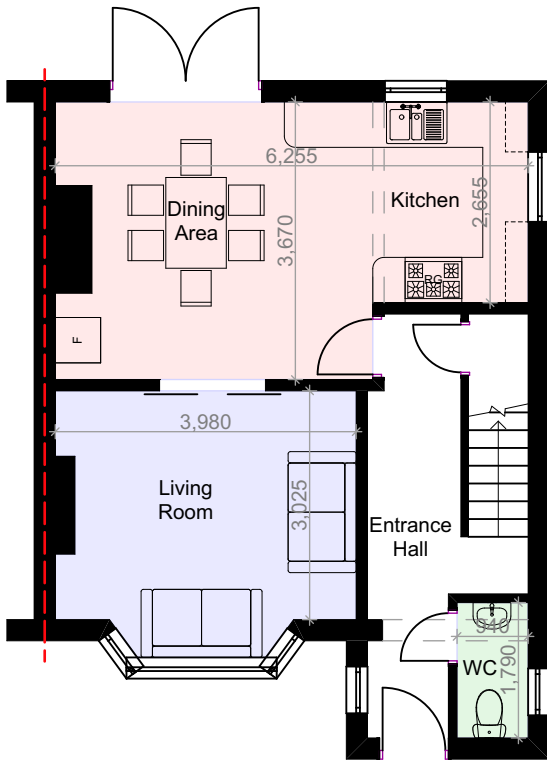
EXISTING GA GROUND FLOOR PLAN
