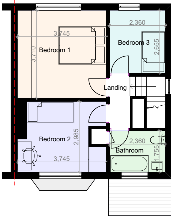
EXISTING GA FIRST FLOOR PLAN
