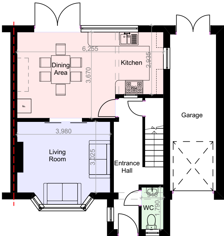
PROPOSED GA GROUND FLOOR PLAN
