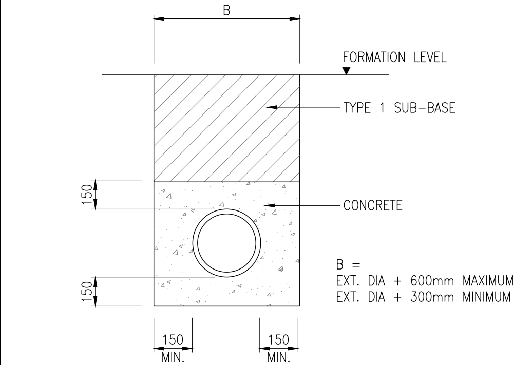
DETAIL OF CLASS 'Z' CONCRETE SURROUND (FOR PIPES UNDER TRAFFICKED AREAS WITH <1.2m COVER)
