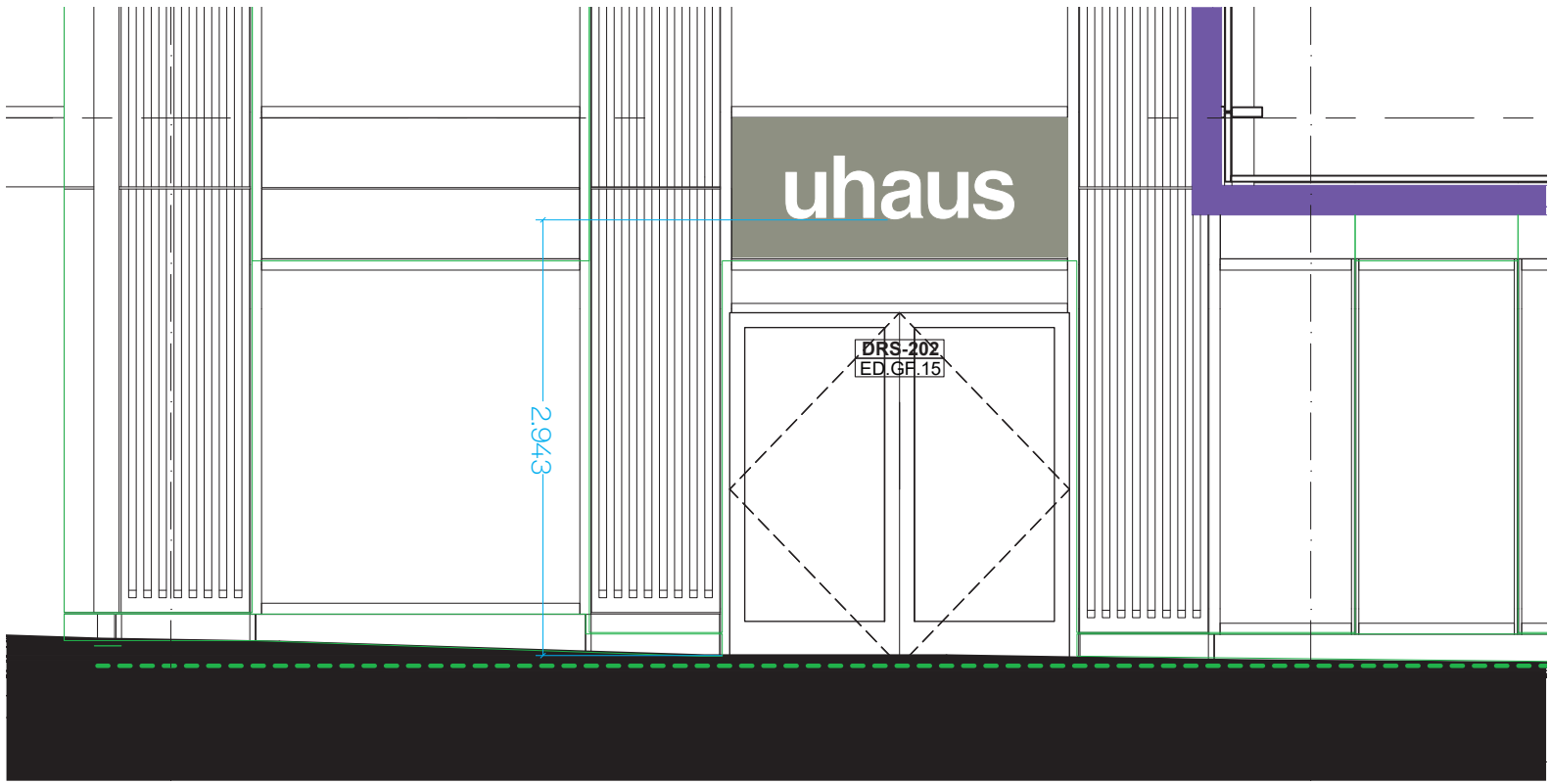
Vita East - Arcade North Elevation 1:50 @ A3
