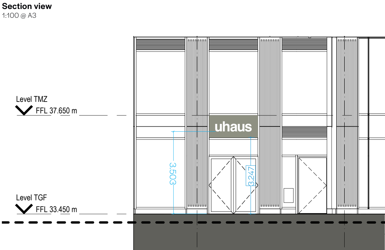
Vita North - South Elevation Symphony Park 1:100 @ A3
