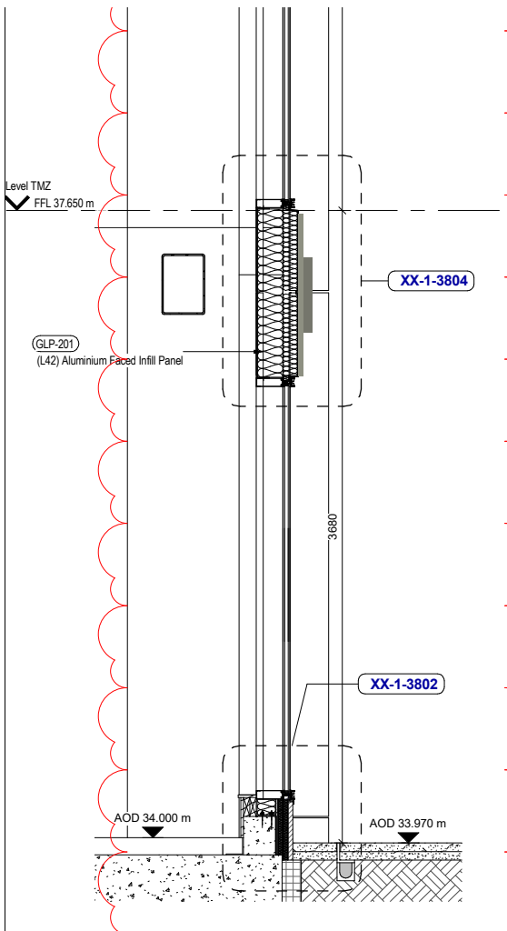
Typical Section View 1:40 @ A3
