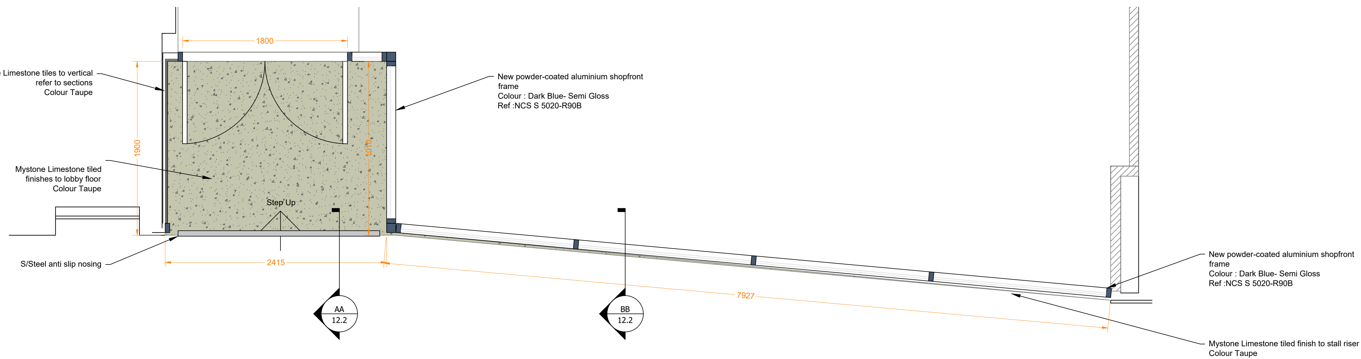
12 Cross Street Elevation Scale: 1:25@A1
