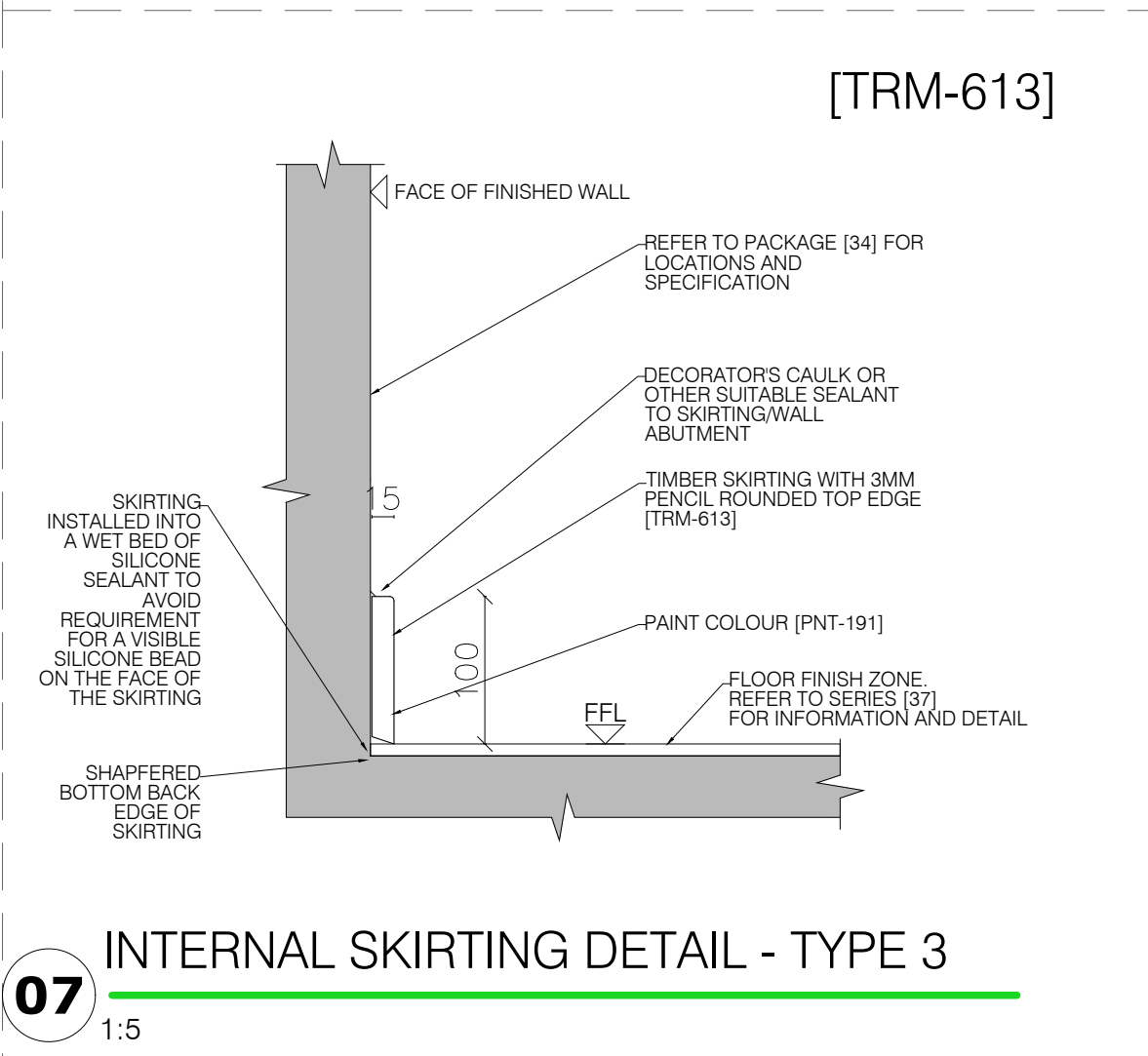
07 INTERNAL SKIRTING DETAIL - TYPE 3
