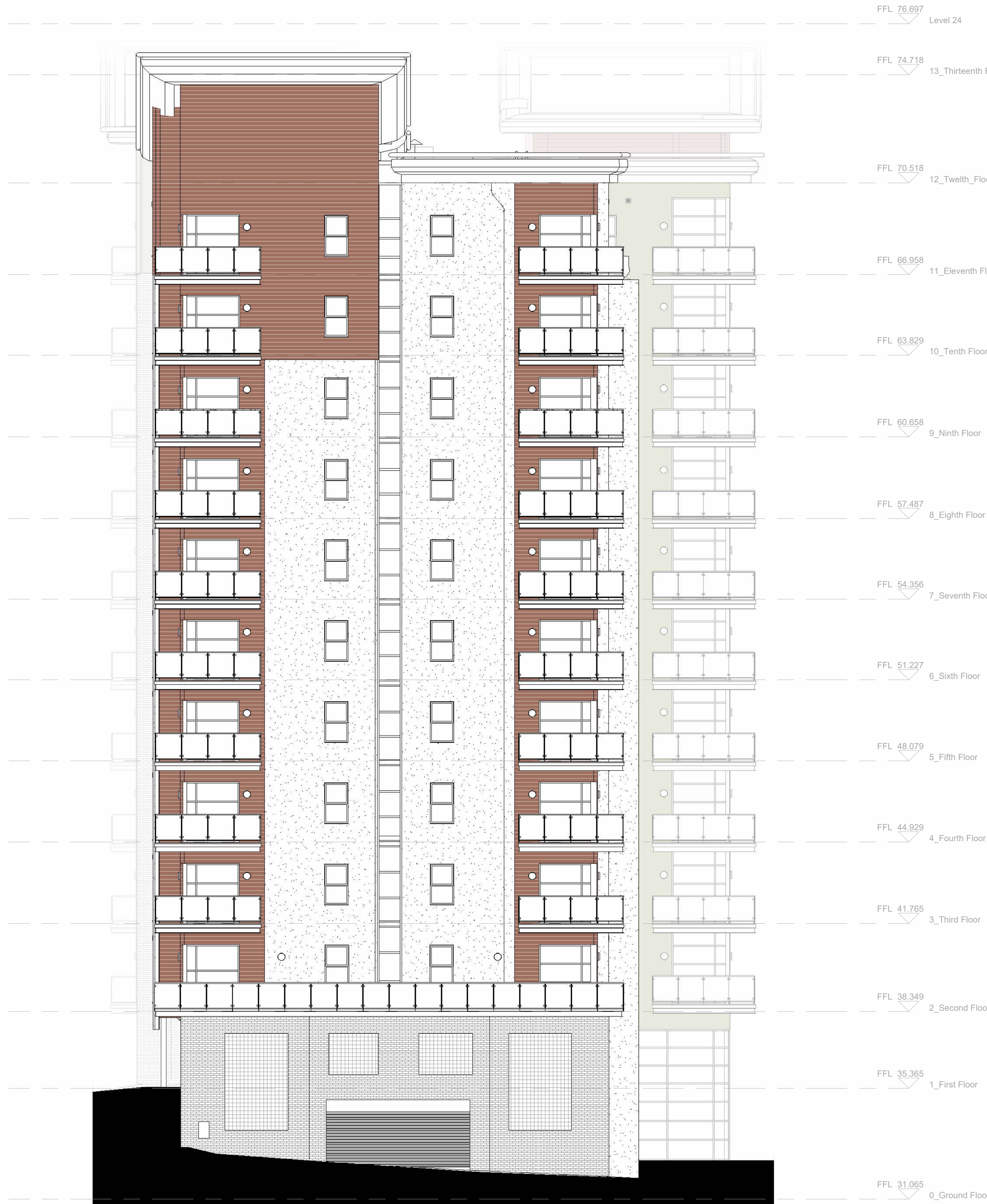
2 ELEVATION SOUTH - REMEDIATION MARK-UP Copy 1 1:100
