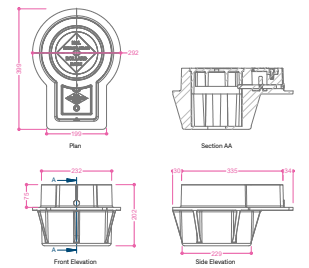
NAL - X-Last series composite socket
