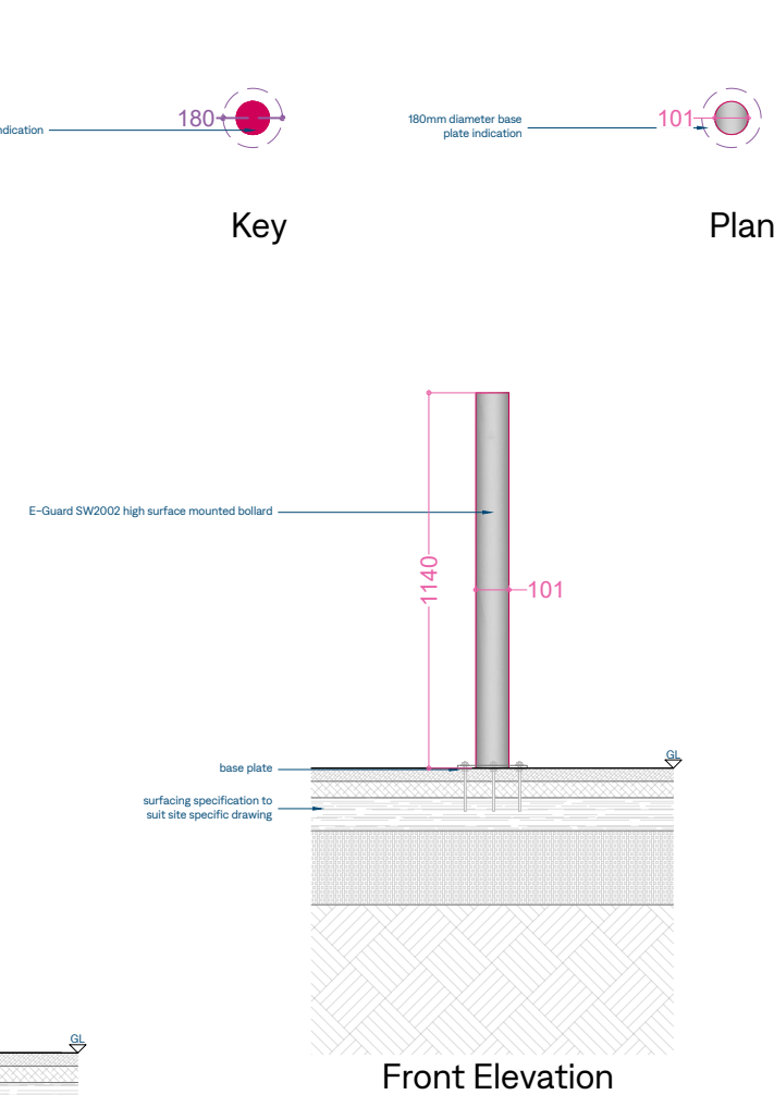
E-Guard - Stainless steel surface mounted bollard
