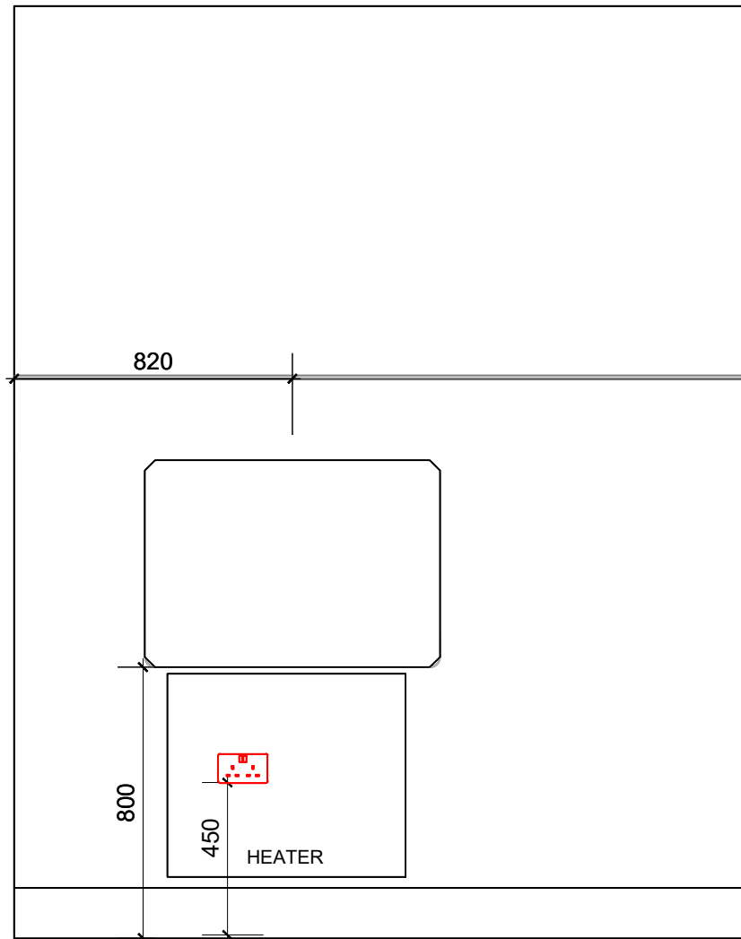
ELEVATION C SCALE 1:20
