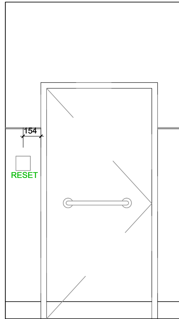
ELEVATION D SCALE 1:20
