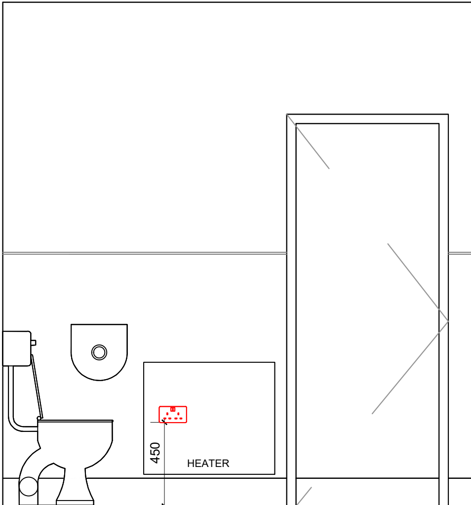
ELEVATION I SCALE 1:20
