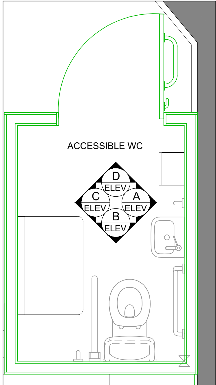
ACC.WC - RREFERENCE PLAN SCALE 1:50
