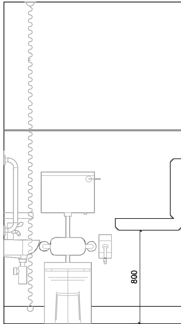
ELEVATION B SCALE 1:20
