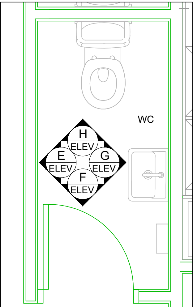
BASEMENT WC - RREFERENCE PLAN SCALE 1:50
