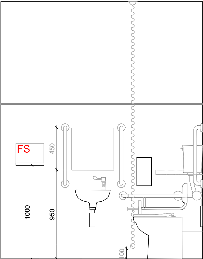
ELEVATION A SCALE 1:20
