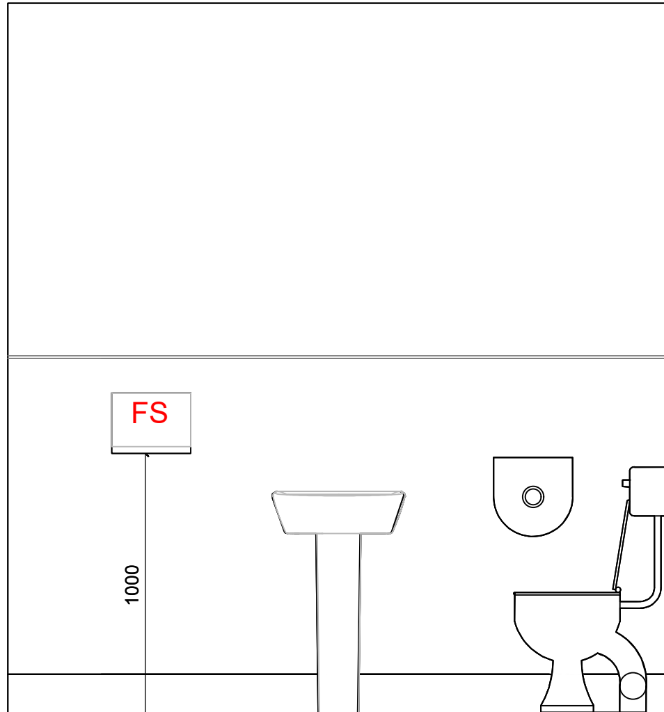
ELEVATION K SCALE 1:20
